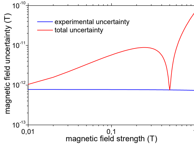
Fig. 2. Uncertainty in the measurement of magnetic field strength by Zeeman spectroscopy of the (v,L,F,S,J,J_z)=(0,0,1,2,2,-2)\rightarrow(0,2,1,2,4,0) transition of \text{HD}^+ . Total uncertainty of the magnetic field (red line) and contribution from the frequency measurement uncertainty (blue line).
