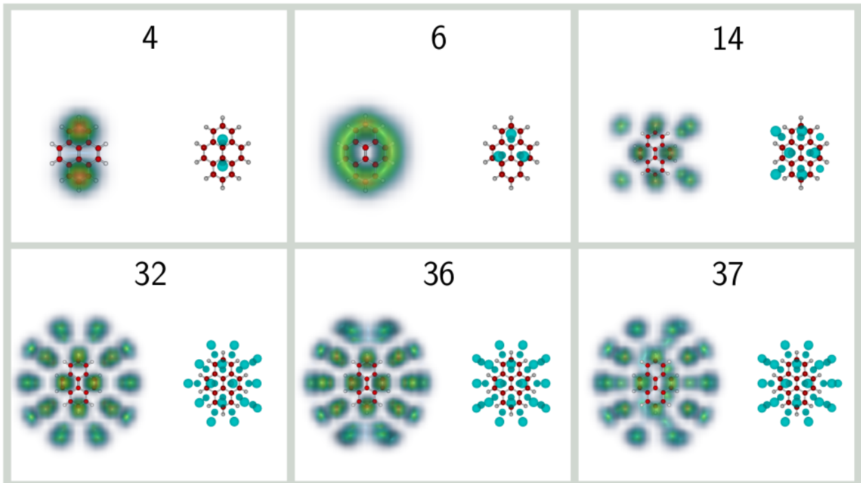
Figure 9: Selected structures of \text{He}_n\text{Pyr}^+ clusters with n = 4, 6, 14, 32, 36, and 37 . For each size, the classical global minima are shown on the right, while the helium densities obtained from the PIMD simulations are shown on the left.
