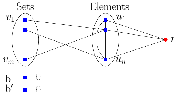
Figure 2: Reduction from SET COVER to RED-BLUE SEPARATION of Theorem 1. Vertex r is red, the others are blue.
