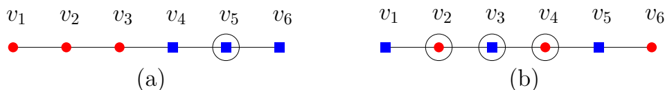
Figure 1: A path of 6 vertices where (a) \text{sep}_{\text{RB}}(P_6, c) = 1 and (b) \text{max-sep}_{\text{RB}}(P_6) = 3 . The square vertices are blue, the round ones are red; the members of the red-blue separating set are circled.
