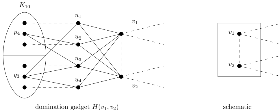
Figure 11: A domination gadget on vertices v_1 and v_2 and its schematic representation.
