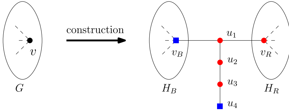
Figure 3: Reduction from DOMINATING SET to RED-BLUE SEPARATION of Theorem 2. Vertices v_B and u_4 are blue, the others are red.
