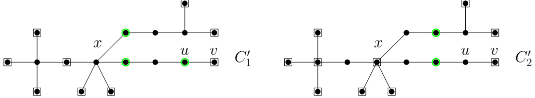
Figure 10: Comparison of the sets C'_1 and C'_2 where the vertices highlighted in green belong to the sets C'_1 \setminus (L(T) \cup S_+(T) \cup NS_3(T)) and C'_2 \setminus (L(T) \cup S_+(T) \cup NS_3(T)) , respectively.
