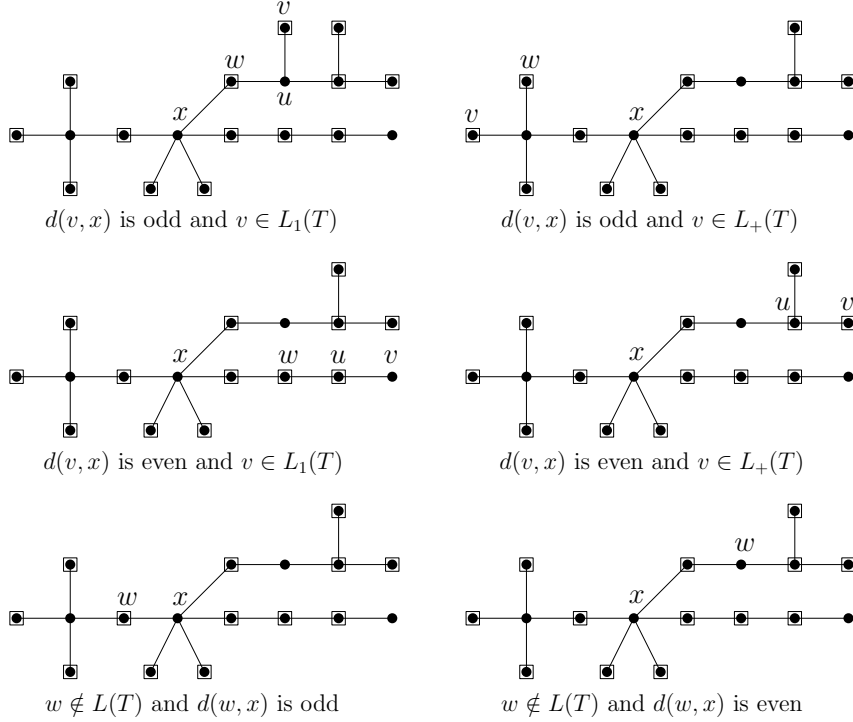
Figure 9: Illustration of various cases for C_1 in Claim 17.1.
