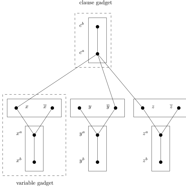
Figure 12: Variable and clause gadgets.
