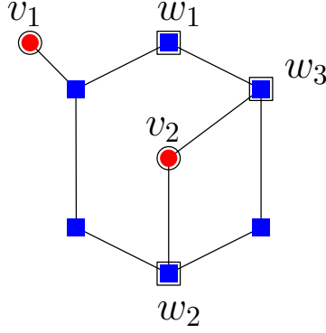
Figure 6: Illustration of Proposition 5: here v_1 has just one blue neighbor hence w_1 is added in S . v_2 's neighbors w_2 and w_3 are also included in S . The square vertices are blue, the round ones are red.
