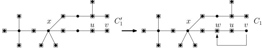
Figure 8: Construction of C_1 from C'_1 where the boxed elements represent members of the set.
