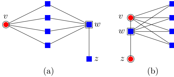
Figure 7: Illustration of Proposition 6: the two cases when the vertices v and w are (a) not adjacent and (b) adjacent. The square vertices are blue, the round ones are red.
