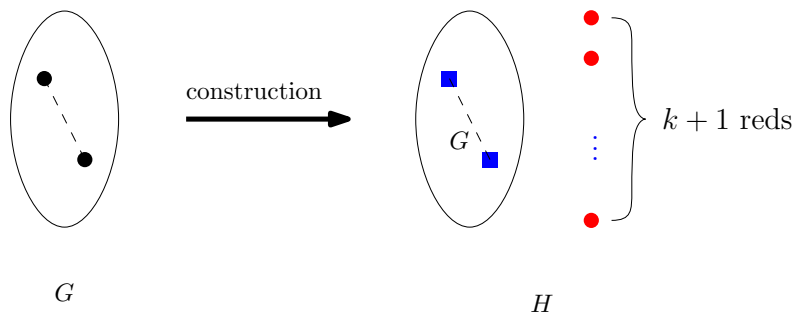
Figure 4: Construction from an instance of DOMINATING SET to an instance of RED-BLUE SEPARATION where size of the smaller color class is bounded. The square vertices are blue, the round ones are red.
