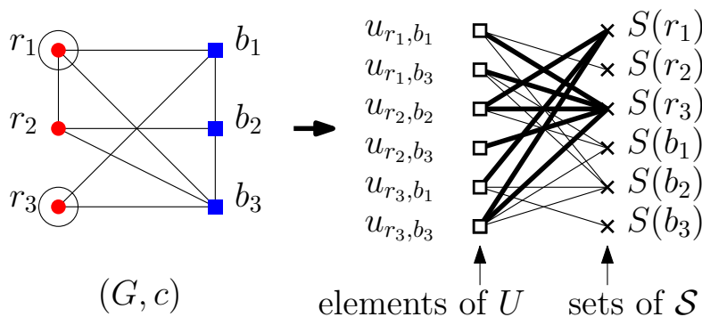
Figure 5: A reduction instance from RED-BLUE SEPARATION of (G, c) (where the square vertices are blue, the round ones are red) to SET COVER of (U, \mathcal{S}) . The separating set in the colored graph (G, c) and the corresponding set cover in the set system (U, \mathcal{S}) has been highlighted.
