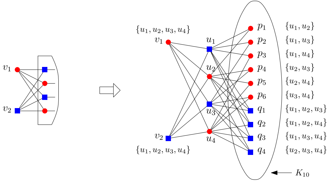
Figure 13: An example to show the reduction from 3-SAT-2L to MAX RED-BLUE SEPARATION. The square vertices are blue, the round ones are red.
