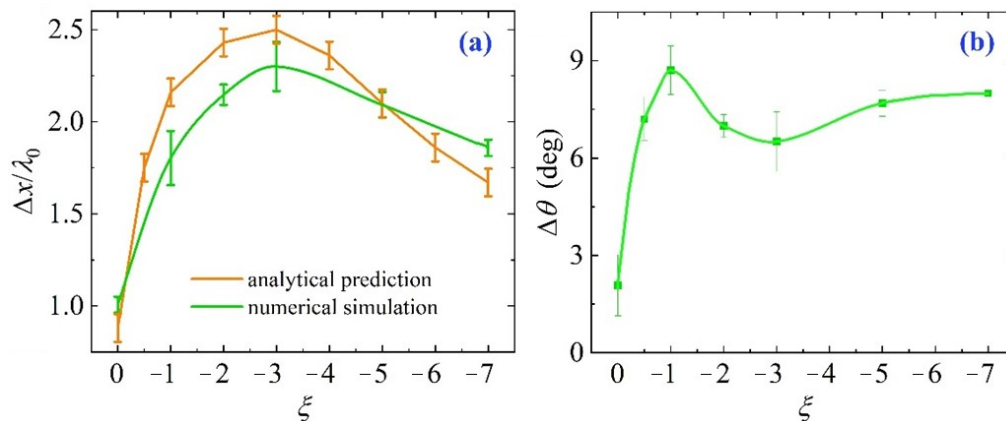
Fig. 2. Panel (a) represents a comparison of the results of numerical simulation (green curve) and analytical calculation (orange curve) of the lateral shift \Delta x / \lambda_0 of the more intense reflected beam in dependence with the phase modulation parameter -7 \leq \xi \leq 0 . Panel (b) shows the angular shift \Delta \theta of the same reflected beam for the same set of values \xi obtained by numerical simulation.
