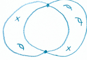
FIGURE 2. An example of branch point of the extension (13) with (g, n) = (4, 2) . The Dehn twist around the two curves of the curve system acts trivially on \bar{\mathcal{S}}_{4,2} and the depicted boundary point of \mathcal{S}_{4,2^*} but non-trivially in the neighbouring points outside the boundary
