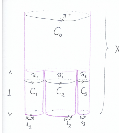
FIGURE 1. The surface with boundary X^+
