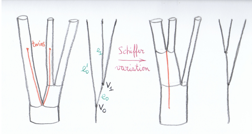
FIGURE 5. Graph changes when a zero moves upward.
