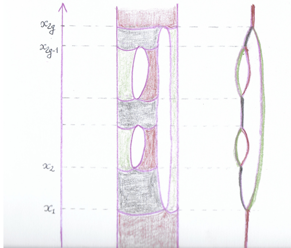
FIGURE 4. An example of the graph of cylinders
