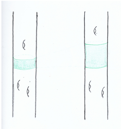
FIGURE 3. Isoperiodic stretching of a cylinder by appropriate Schiffer variations
