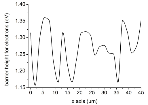
Fig. 5. Example of barrier height distribution as a function of x axis for electrons. The distribution is calculated as being in the range \pm 10\% of the optimized value presented in Table 1.
