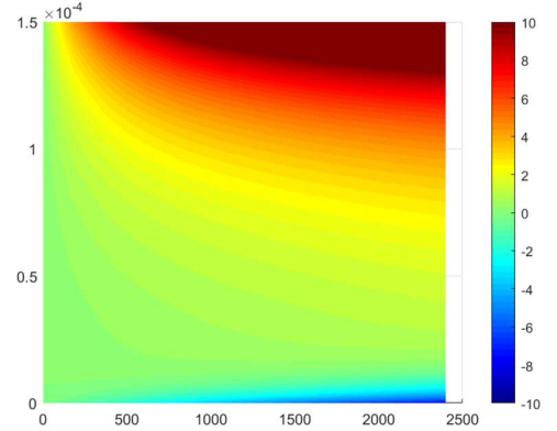
Fig. 2. Net charge density cartography as a function of time and depth in the sample ( y ) when only Schottky injection is considered. Horizontal axis: time in s. The colour scale provides charge density in C/m^3 .
