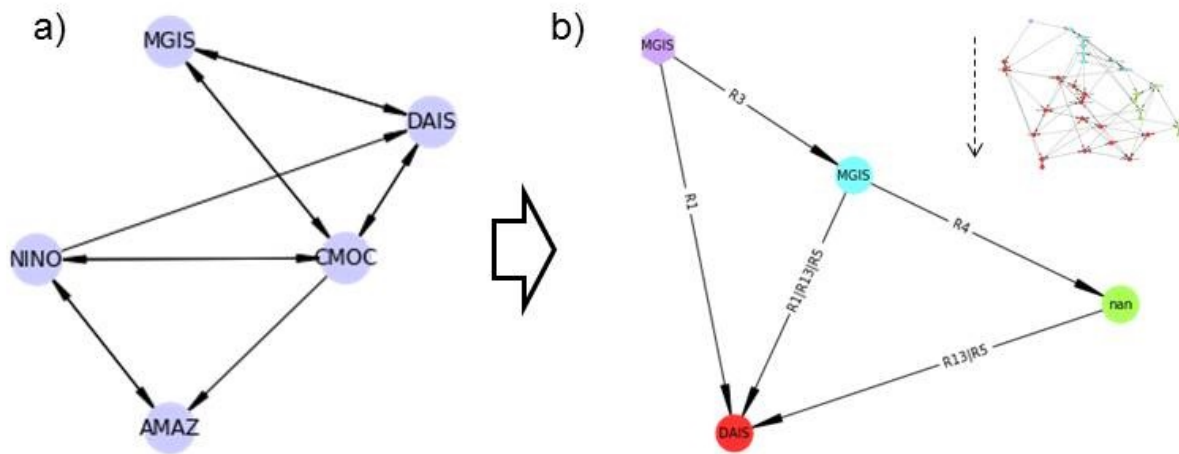
Figure 1. The interaction network (a) made up of the main TPs identified and discussed in (2, 7), with its computed state-transition space displayed in reduced/merged (b) and extended versions (insert). The interaction network displays state variables (a, nodes) and interacting processes (a, edges). The resulting state-transition space displays qualitative stabilities (b, nodes) with systematically present TPs (b, node labels) and event transitions (b, edges labeled R_x ) connecting them (4). These possibilistic spaces highlight the potential tipping cascades, absent here (i.e. a single TP in each stabilities), yet still with highly incomplete Earth modeling.
