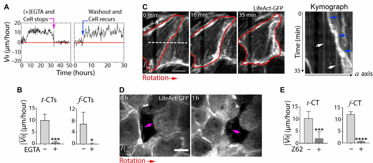
Fig. 5. Roles of cell-cell adhesions and cell polarity in rotating CTs. (A) Graphs showing EGTA treatment ceased CeR ( V_0 \approx 0 ; magenta arrow) and CeR recurrence (blue arrow) after washout. (B) Plots presenting |V_0| for different rotating CTs before and after EGTA treatment ( n=4 for all cases). (C) 2D time-lapse (15 s per frame) projections demonstrating actin dynamics of a t -CT ( \varnothing = 100 \mu\text{m} ) expressing LifeAct-GFP during CeR. The cell periphery is drawn in red. The kymograph on the right was obtained by reslicing along white dashed line (0 min). White arrows indicate trajectories of immobile long-range actin filaments, and blue arrows show displacement of cell front with respect to a axis. (D) 2D time-lapse projections demonstrating actin-based cryptic protrusion of a rotating t -CT ( \varnothing = 100 \mu\text{m} ) consisting of WT and LifeAct-GFP MDCKs. Magenta arrows denote lamellipodial protrusions of a LifeAct-GFP-expressing cell toward a WT (unmarked) cell. (E) Graphs presenting |V_0| for different rotating CTs before and after Z62 treatment ( n=6 for t -CTs and n=3 for f -CTs). Student's t test, *P < 0.05 , ***P < 0.001 , and ****P < 0.0001 . In (B) and (E), data are presented as means \pm SD. Red arrows indicate rotation direction. Scale bars, 20 \mu\text{m} .
