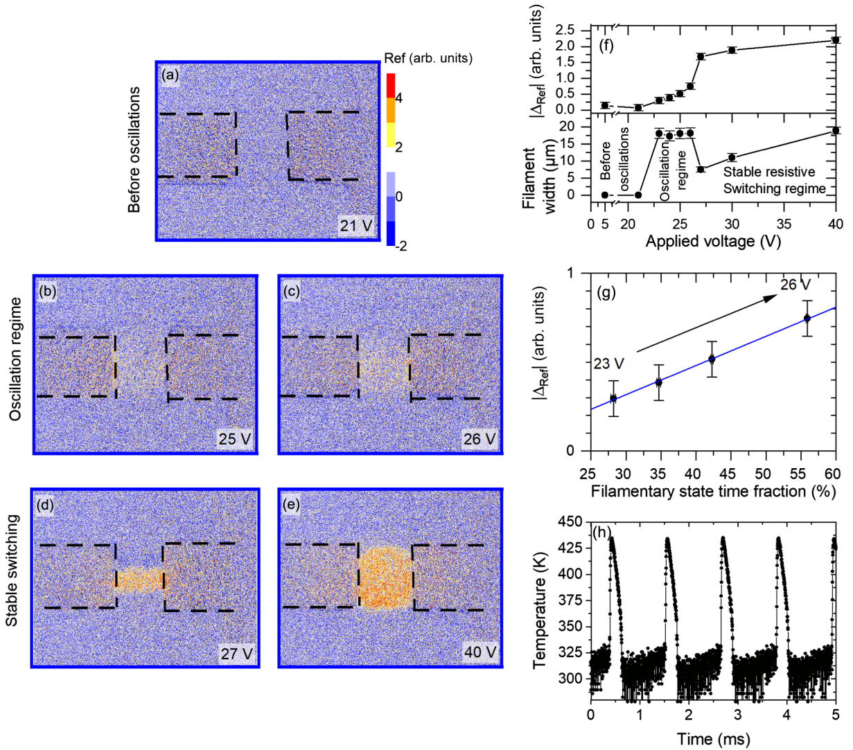
FIG. 4. Optical imaging of the self-oscillation regime in V_3O_5 . (a)–(e) Differential contrast images of the resistive switching in V_3O_5 acquired at different voltages, corresponding to the homogeneous regime before oscillations in (a), the oscillation regime in (b) and (c), and during the stable resistive switching regime after the oscillations in (d) and (e). The low-temperature phase is in blue, and the high-temperature phase is in orange. The appearance of a wide low-intensity filament can be seen in the oscillation regime. (f) Applied voltage dependence of the maximum intensity and width of the filament. (g) Intensity of the reflectivity change vs time fraction spent in the filamentary state during the oscillation regime. The time spent in the filamentary state is extracted from the electrical measurement for each voltage (see Supplemental Material [46] for details). (h) Temperature vs time extracted from time-resolved IR measurements in the self-oscillation regime. The temperature changes between 325 and 430 K each oscillation cycle.
