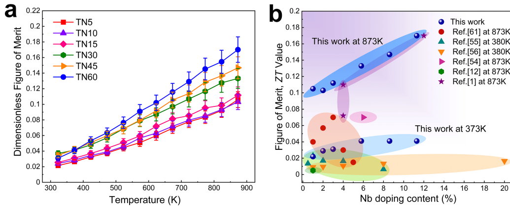
Figure 11. Thermoelectric figure for rutile-based ceramics: (a) results from this study ( ZT ) as a function of temperature; (b) compilation of ZT values for single Nb-doped, \text{TiO}_2 -based thermoelectric ceramics.
