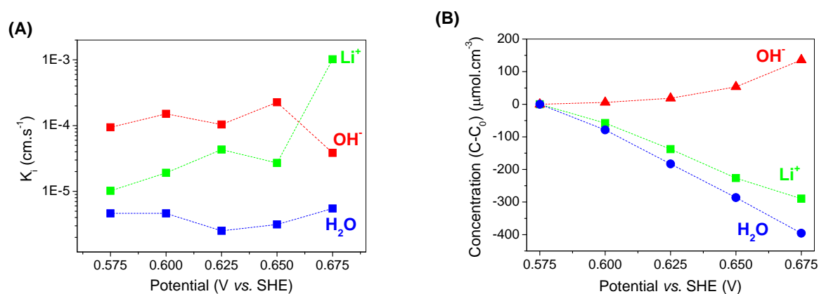
Figure 6: Ac -electrogravimetric results. (A) Kinetics parameters K_i of Li^+ , OH^- and H_2O vs. the applied potential of Ni/Fe-LDH. (B) Relative concentration variations, C_i-C_0 , of Li^+ , OH^- and H_2O transferred to the Ni/Fe LDH-coated Au electrode vs. the applied potential. Electrolyte: 1 M LiOH.
