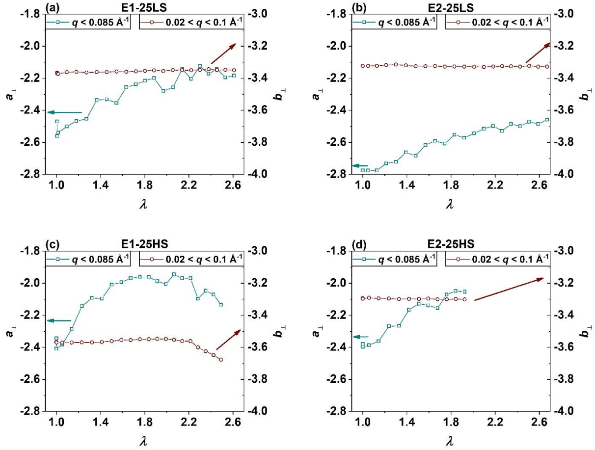
Figure 9. The exponent a_{\perp} in the equatorial direction is determined in the low- q region and b_{\perp} in the high- q region for (a) E1-25LS (b) E2-25LS (c) E1-25HS and (d) E2-25HS.
