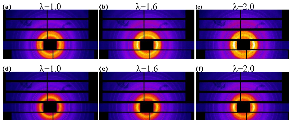
Figure 3. 2D-WAXS patterns of E1-35LS under different mechanical strains: \lambda = 1.0 (a), 1.6 (b) and 2.0 (c). 2D-WAXS patterns of E1-25HS at \lambda = 1.0 (d), 1.6 and 2.0 (f) with a crosshead speed of 10 mm/min.
