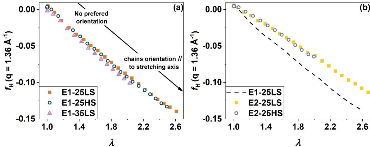
Figure 5. The apparent Herman’s factor f_H was calculated for WAXS in situ during tensile testing at q=1.36 \text{ \AA}^{-1} for (a) E1-25LS, E1-25HS and E1-35LS (b) the comparison of EPDM orientation for composites with matrix 1 and matrix 2 and as a function of CB structure during stretching where E1-25LS is symbolized by dotted line (the orientation is superposed for the other composite as shown in Figure 5a).
