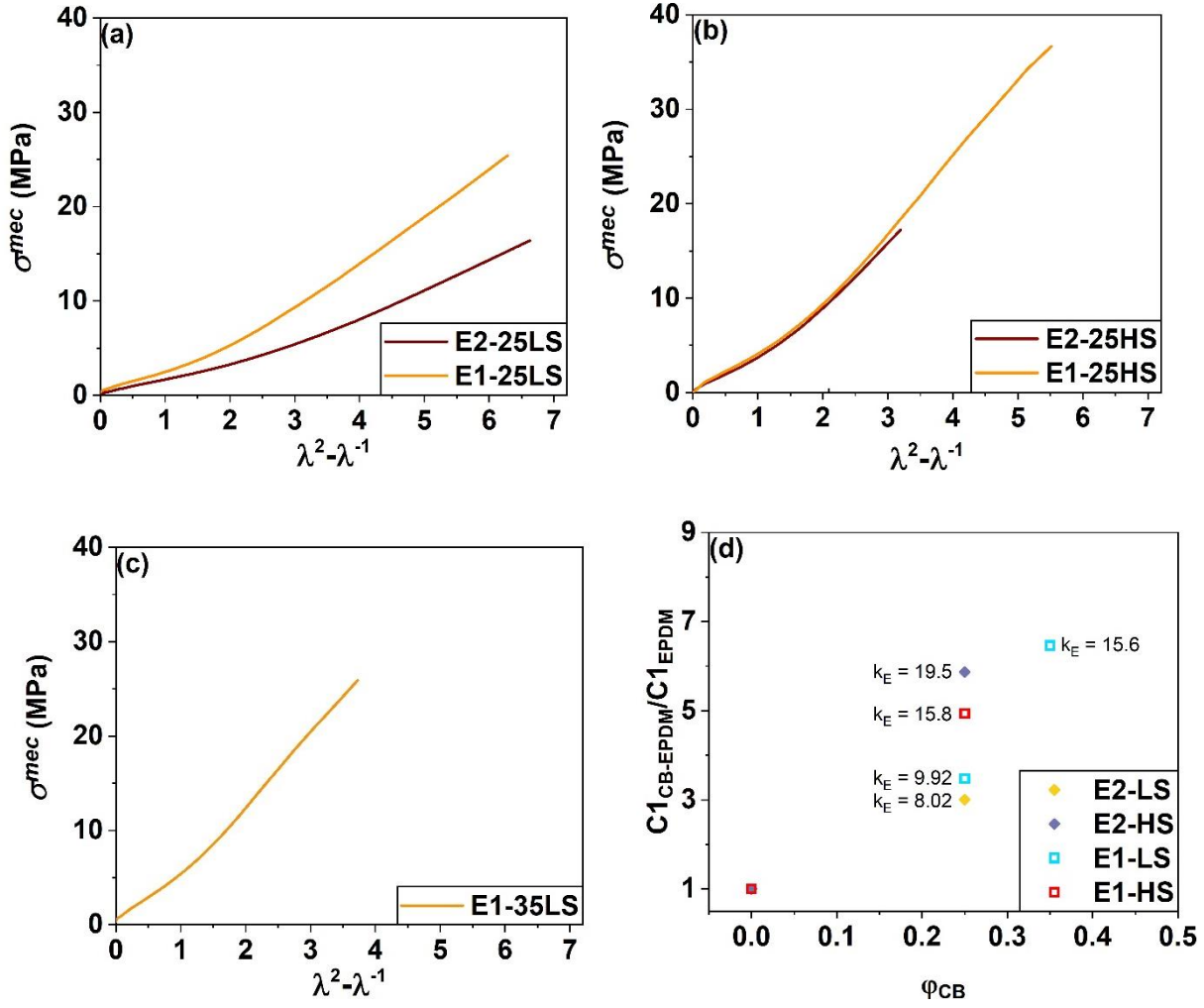
Figure 6. Impact of the EPDM matrix, CB content and CB structure on \sigma^{mec} - (\lambda^2 - \lambda^{-1}) curves for: (a) E1-25LS and E2-25LS; (b) E1-25HS and E2-25HS; (c) E1-35LS. (d) Corresponding parameter C1 = G/2 for each system is determined and normalized by the parameter C1 of E1-0 or E2-0. The values of the Einstein coefficients are reported for each composites
