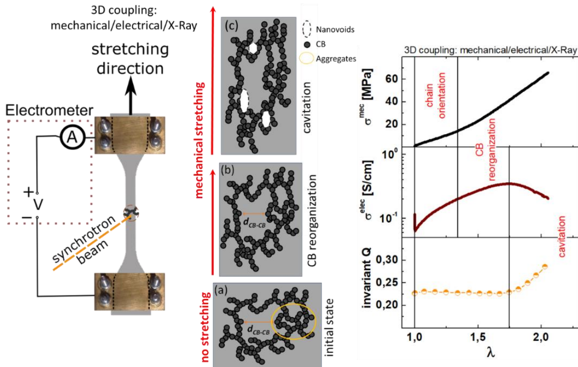
Figure 13. Scheme of microstructural mechanisms observed with Electrical/Mechanical/X-Ray coupling. The application of stress/strain is related to EPDM orientation, the increase of conductivity is correlated with CB lateral interpenetration and decrease of conductivity is due to cavitation during tensile test.
