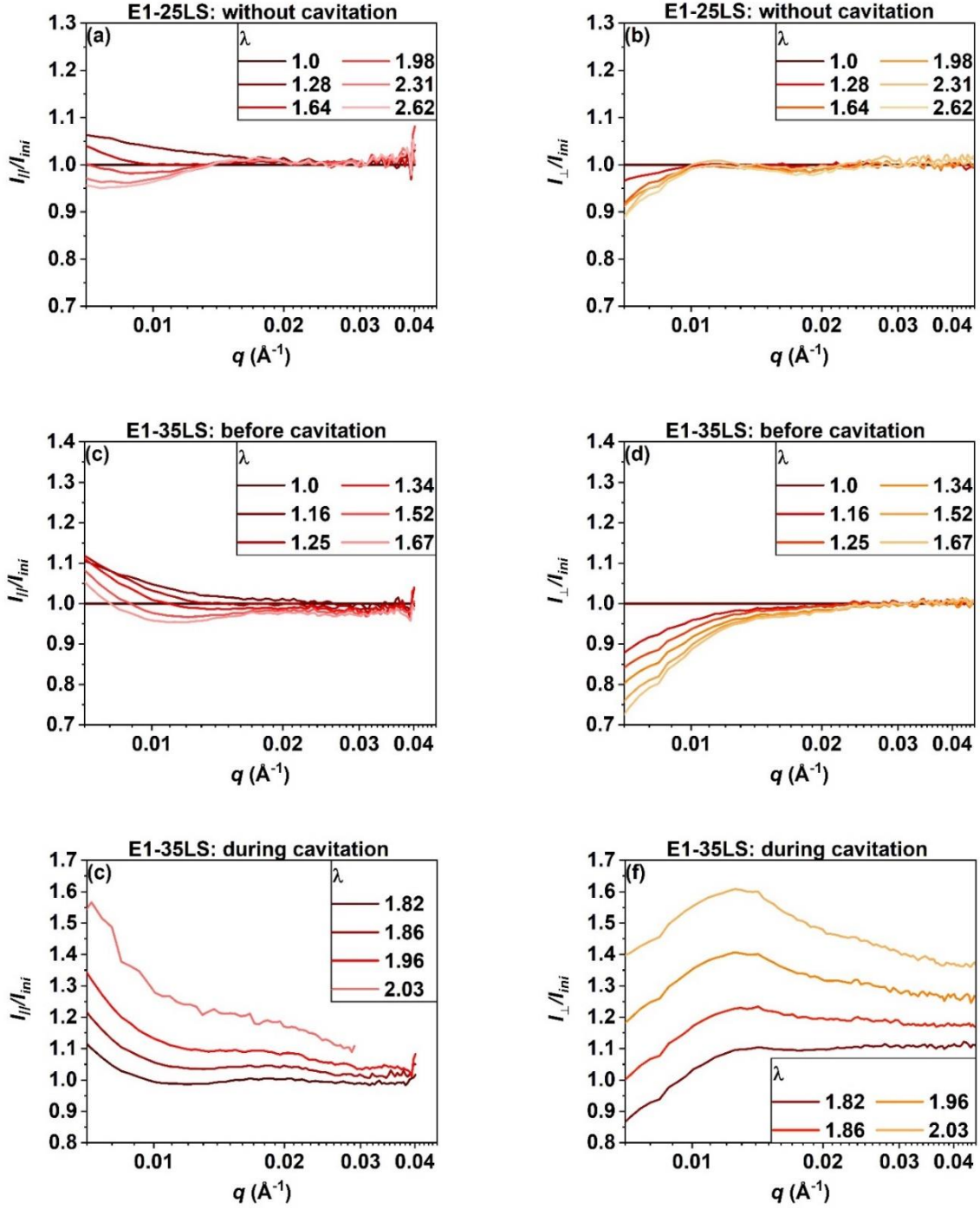
Figure 11. Evolution of Intensity ratios (a) \frac{I_{||}(q)}{I_{ini}(q)} (b) \frac{I_{\perp}(q)}{I_{ini}(q)} for E1-25LS, which is uniaxial stretched without cavitation. Evolution of the ratio (c) \frac{I_{||}(q)}{I_{ini}(q)} (d) \frac{I_{\perp}(q)}{I_{ini}(q)} for E1-35LS during uniaxial stretching before cavitation and (e) \frac{I_{||}(q)}{I_{ini}(q)} (f) \frac{I_{\perp}(q)}{I_{ini}(q)} for E1-35LS during cavitation.
