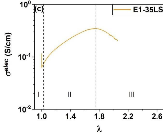
Figure 7. Influence of EPDM matrix, CB content and CB structure on the electrical properties under large elongation for (a) E2-25LS and E1-25LS (b) E2-25HS and E1-25HS (c) E1-35LS.
