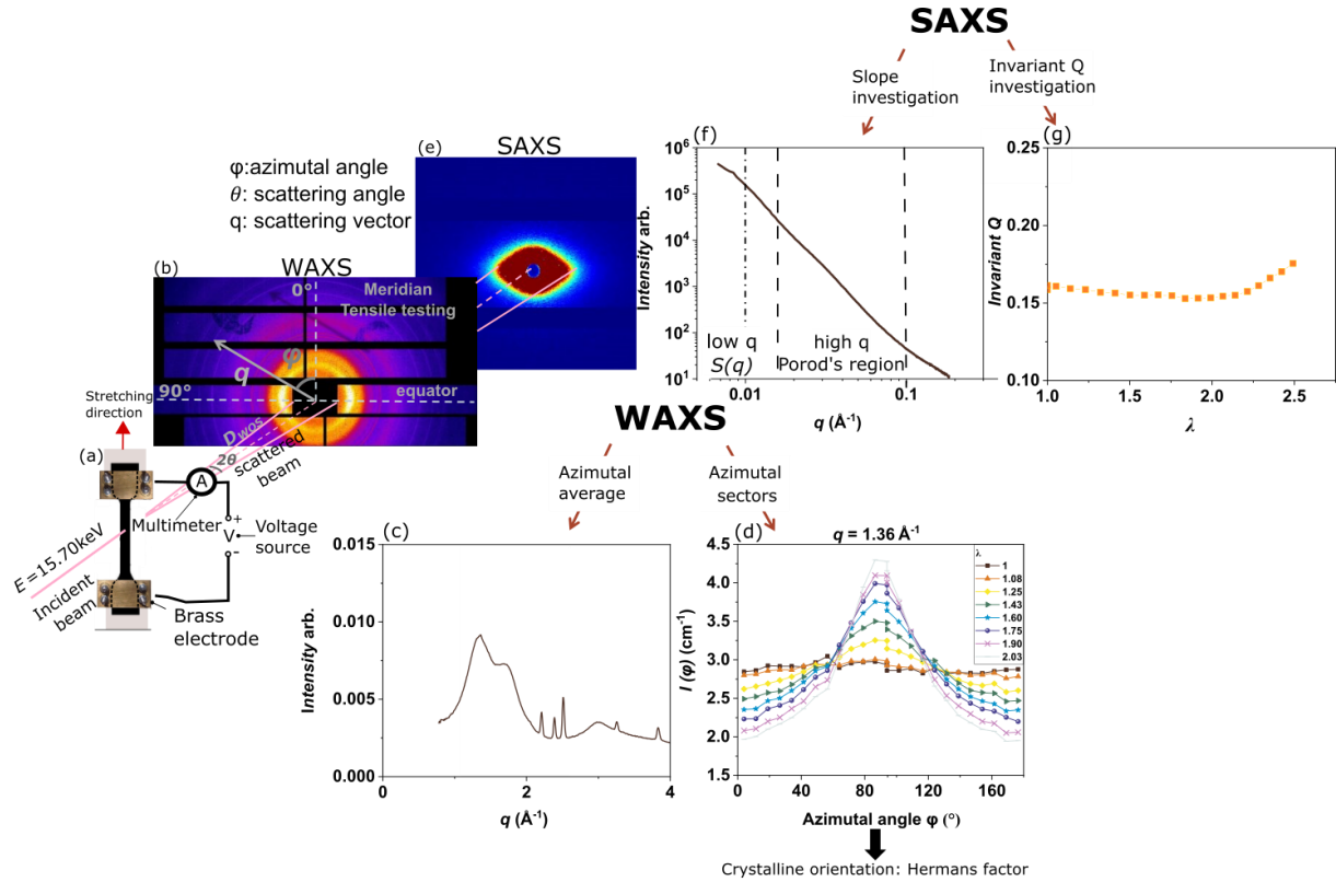
Figure 1. (a) Schematic representation of the coupled mechanical/electrical/structural investigations (b) 2D WAXS pattern, in which each pixel is characterized by an intensity I , a scattering angle 2\theta (corresponding to a diffusion vector q ) and an azimuthal angle \phi (c) Analysis of a WAXS diffractogram obtained by azimuthal average of the intensity for each q . (d) The molecular orientation of polymer chains is observed by division of the WAXS pattern in azimuthal sectors. (e) 2D SAXS pattern, in which each pixel is characterized by an intensity I , corresponding to a scattering vector q and an azimuthal angle \phi . (f) SAXS curves obtained for EPDM filled with CB could be divided in two regions. (g) Scattering invariant Q evolution with elongation ratio \lambda .
