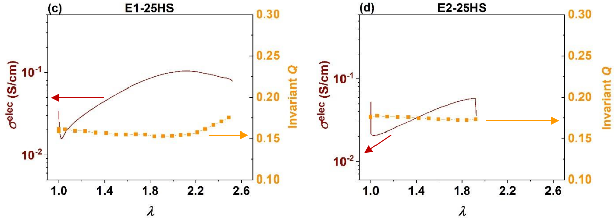
Figure 10. Correlation between electrical conductivity \sigma^{elec} and the scattering invariant Q with increasing extension ratio \lambda for (a) E1-25LS (b) E1-35LS (c) E1-25HS and (d) E2-25HS. Fracture occurs before cavitation in the E2-25HS composite, where crosslinking is possibly too low to induce cavitation under deformation. Cavitation occurs in E1-35LS and E1-25HS and manifests as an increase in the Q values at large extension ratios.
