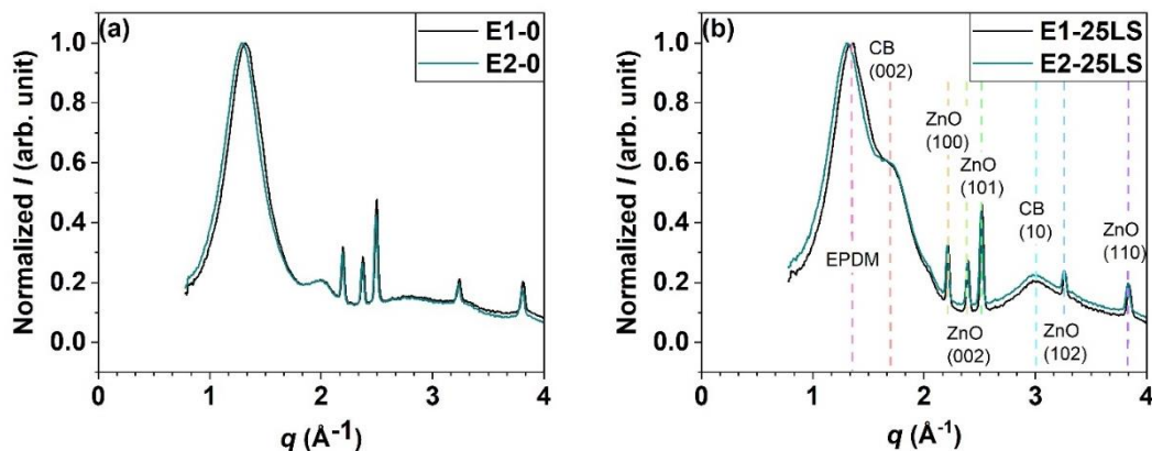
Figure 2. WAXS patterns of (a) unfilled E1-0 and E2-0 composites (b) filled E1-25LS and E2-25LS composites.
