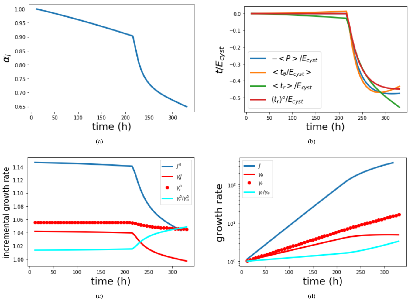
FIG. S2: Time evolution of several computed quantities in Experiment 2. (a) : Evolution of the angular elastic deformation gradient at the inner surface of the cyst \alpha_i . (b) : The mean radial, the ortho-radial stresses and the stress invariant \langle t_r \rangle , \langle t_\theta \rangle , -\langle P \rangle as well as the radial stress at the outer surface (t_r)_o normalized by E_{cyst} . Those values contribute to explain the buckling instability at the end of the experiment. (c,d) : Evolution of the different incremental (c) and total (d) growth variables J = \gamma_\theta^2 \gamma_r , \gamma_\theta , \gamma_r , \gamma = \gamma_r / \gamma_\theta with time.
