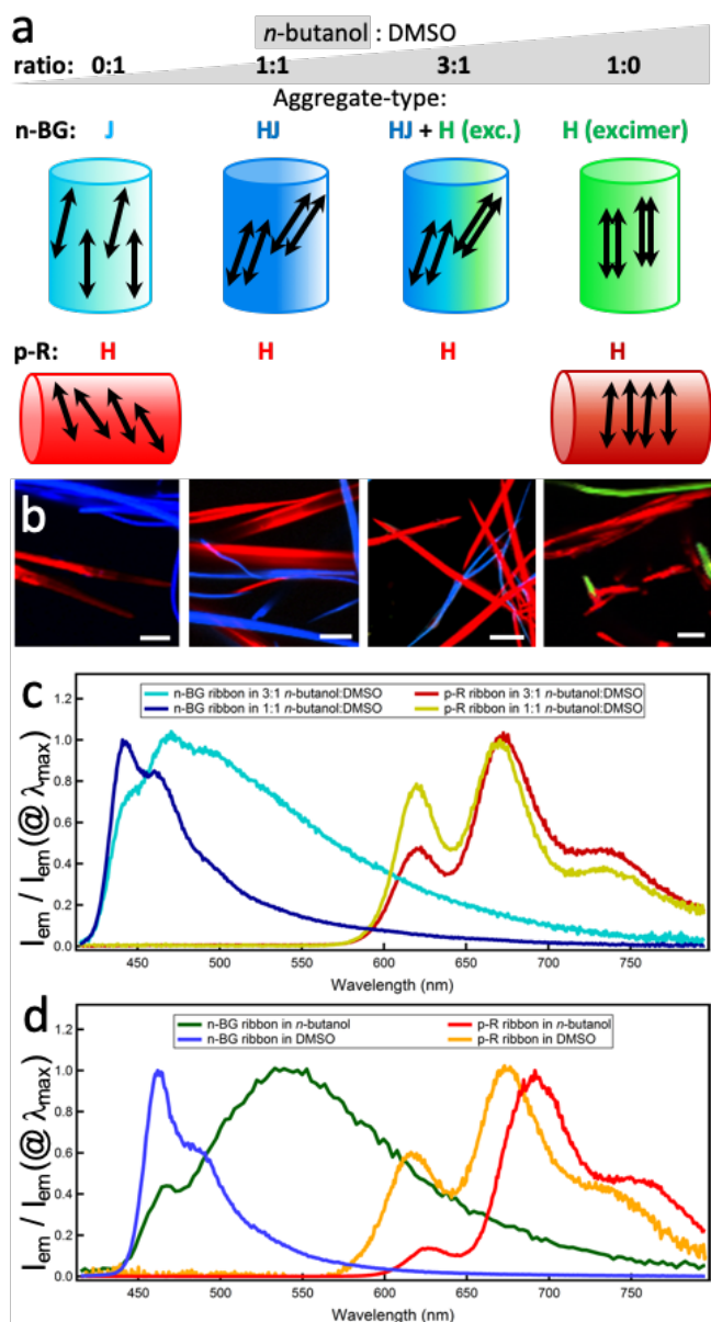
Figure 2. a) Solvent mixtures for a) and b). Attributions of the main emission features to the aggregate types and simplified representation of possible packing within a ribbon of four molecules (each represented by the emission dipole oriented along the short axis of the n -acene, additional symmetry is probable). b) Hyperspectral images of self-sorted ribbons in the four solvent conditions. Red-emissive ribbons are attributed to p-R , the other to n-BG (Scale bars: 5 \mu\text{m} ). c) and d) Relative emission intensity spectra of each ribbon type in the four solvents conditions; spectral data taken from the ribbons of the hyperspectral images b). \lambda_{\text{ex}} = 375 \text{ nm} .
