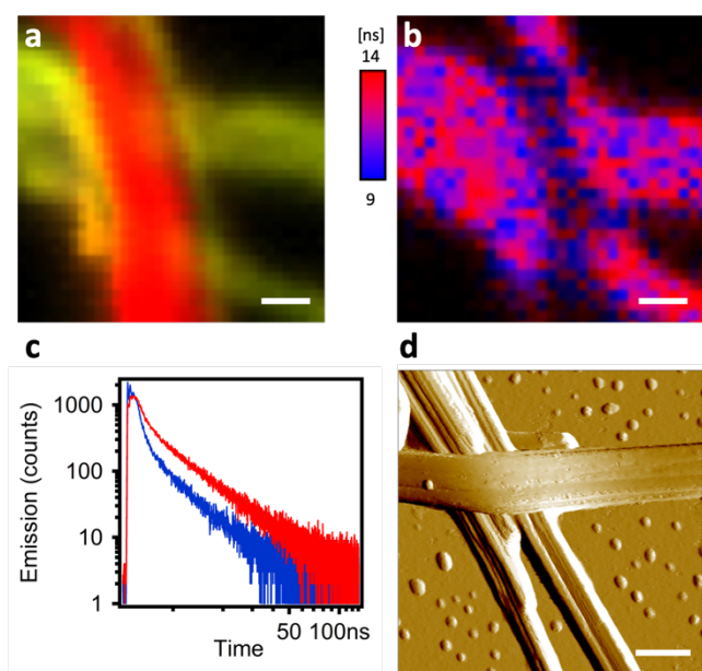
Figure 4. a) Hyperspectral image of a n-BG / p-R ribbon p-n-junction grown in n -butanol (scale bars: 500 nm). b) FLIM (average fluorescence lifetime) image using a 510/80 bandpass filter to retain n-BG emission only. c) Decays of n-BG emission of an isolated ribbon (red curve) and of the junction in (b) (blue curve). Red decay tri-exponential fit (lifetime \tau and amplitude thereof A ): \tau_1 = 0.6 ns ( A_1 = 21\% ), \tau_2 = 3.4 ns ( A_2 = 60\% ), \tau_3 = 15.9 ns ( A_3 = 19\% ); blue decay: \tau_1 = 0.3 ns ( A_1 = 16\% ), \tau_2 = 1.9 ns ( A_2 = 63\% ), \tau_3 = 10.2 ns ( A_3 = 21\% ). \lambda_{\text{ex}} = 375 nm. d) AFM amplitude image of a p-n-junction grown in n -butanol, deposited and dried on a glass cover slip. The “horizontal” ribbon is n-BG , and the “vertical” ribbon is p-R .
