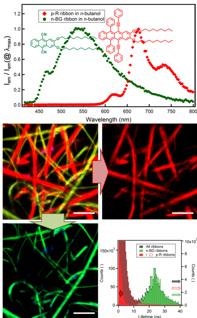
Figure 1. a) Molecular structures of n-BG (green) and p-R (red) and relative emission intensity spectra I_{em}/I_{em}(\lambda_{max}) of the two different nanoribbons in n -butanol. b) Hyperspectral image: the emission spectrum of each pixel is converted into the corresponding RGB-color, \lambda_{ex} = 375 nm. The spectra in a) are obtained from individual ribbons from this map. c) Digital bandpass filter (650 nm - 780 nm) applied on b) highlighting the ribbons attributed to p-R . d) Digital bandpass filter (405 nm - 550 nm) applied on b) showing the ribbons attributed to n-BG . (Scale bar: 5 \mu m). Note: some blue emissive spots can be attributed to photo-oxidized p-R (see S.I.). e) Fluorescence lifetime distribution of the same area: the longer lifetimes are correlated to the green-emissive, and the shorter to the red-emissive ribbons.
