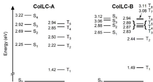
Figure 3. Excited-state energy diagram for ColLC-A and ColLC-B at the T1 geometry.
