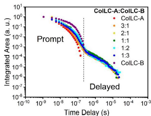
Figure 7. Time-resolved photoluminescence decay curves for ColLC-A, ColLC-B, and blend films at room temperature.
