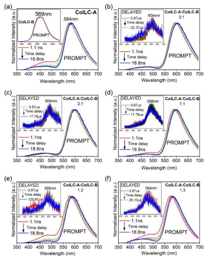
Figure 6. Time-resolved normalized emission spectra of: (a) ColLC-A and ColLC-B (inset). (b-f) Time-resolved normalized emission spectra of blend films, showing the prompt and delayed (insets) regimes. All measurements were performed at room temperature, using a 355 nm excitation source.
