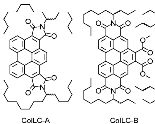
Figure 1. Chemical structures of ColLC-A (left, clearing temperature 265 °C) and ColLC-B (right, clearing temperature 151 °C), which both exhibit a hexagonal columnar mesophase at room temperature and up to the clearing transition.
