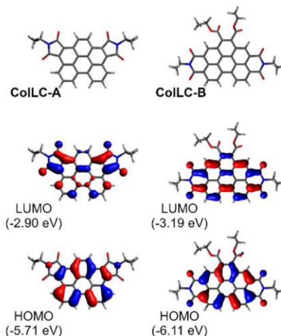
Figure 2. Optimized ground-state geometry (top) and HOMO/LUMO iso surfaces (middle and bottom). Alkyl groups are shortened to isopropyl and ethyl.
