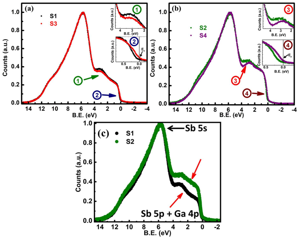
Fig. 8 The valence band structure of samples S1 and S3 (a), S2 and S4 (b) and S1 and S2 (c). The insets (1) and (3) indicate the 'dip' observed during crystallization, and (2) and (4) indicate that the valence band maximum of amorphous samples' lies deeper than the crystalline samples. The enclosed red arrows in (c) indicate the significant rise in spectral intensity observed due to the introduction of nucleation sites.
