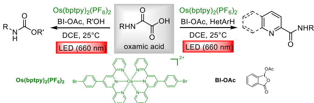
Fig. 1 Decarboxylation of oxamic acids under NIR conditions
