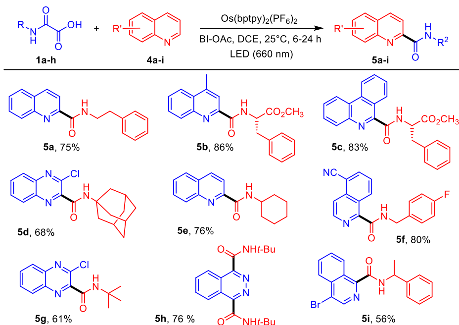
Scheme 2 Os(II)-mediated decarboxylation of oxamic acids in the presence of heteroarenes under NIR irradiation. a Reaction time of 6 h. b Reaction time of 24 h.
