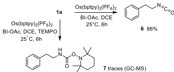
Scheme 3 Trapping experiments.
