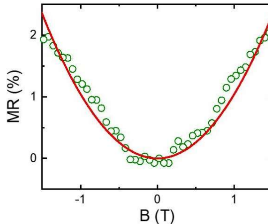
Figure S5. Magnetoconductance measured with the magnetic field in plane, transverse to the current, at 2 K.
