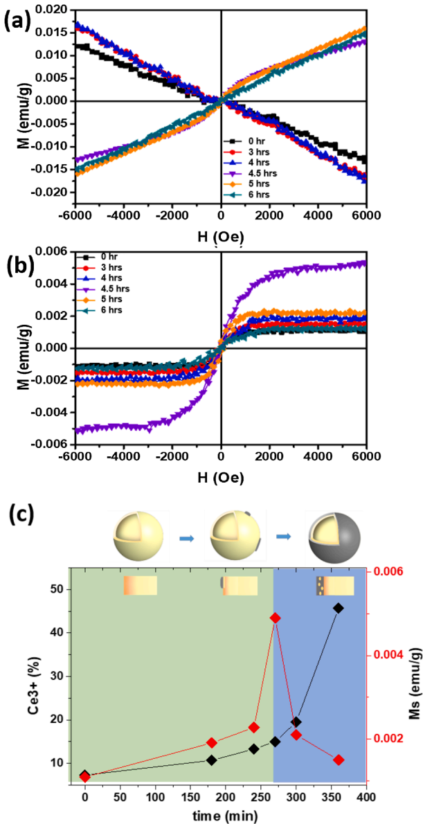
Fig. 6. (a) M–H curves before background subtraction of CeO 2 hollow spheres after reacting with citric acid for different times. (b) M–H curves after the background subtraction. (c) The variation of saturation magnetization, Ms, and Ce 3+ content with the reaction time of the treated samples. The evolution of microstructure with reacting time is illustrated in the insert figure.
