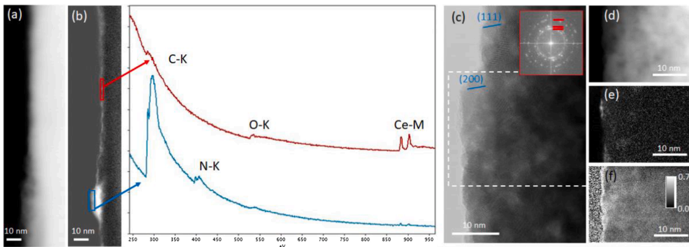
Fig. 4. (a) STEM-HAADF and (b) C-K map and spectra obtained at the surface of the sphere. A heterogeneous layer of carbon is observed, with a thickness of ca. 1–2 nm (spectrum from the red box). Furthermore, it can be observed some thicker carbon part where nitrogen and a small amount of cerium are present (spectrum from the blue box). (c) STEM-BF revealing the surface crystallinity of the ceria sphere. A diffraction pattern is in inset with the red bars indicating (1 1 1), (2 0 0) and (1 1 0) ceria planes (d) STEM-HAADF, (e) EELS C-K map and (f) \text{Ce}^{3+}/\Sigma\text{Ce} map corresponding to the areas boxed in (c). A thin layer of higher \text{Ce}^{3+} is present at the surface but its intensity is modulated by the presence of carbon layer. The intensity scale of the \text{Ce}^{3+}/\Sigma\text{Ce} spans from 0 (black) to 0.7 (white).
