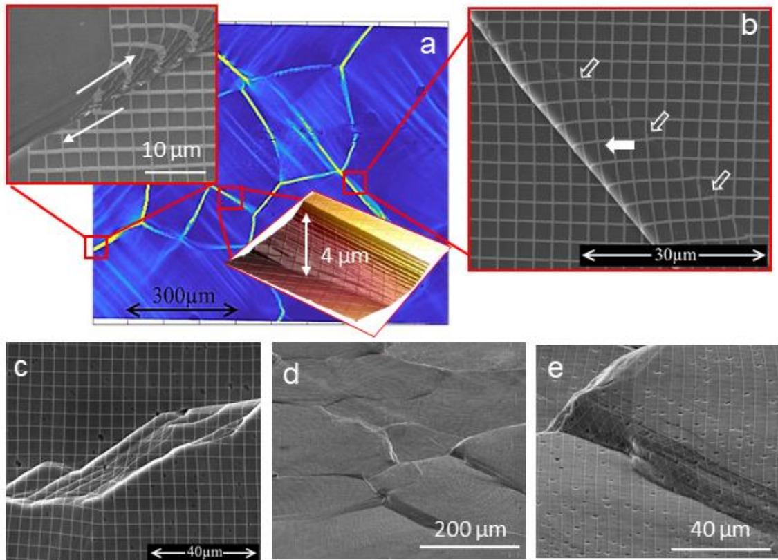
Figure 10: Intense GBS at 300°C (a and b) and 400°C (c, d, e) leads to development of marked topography (a, d and e) and grain boundary migration (b and c). Above 300°C the GBS is so active that the marking grid may be severely distorted/damaged (a). Continuous (b) or step-wise (c) grain boundary migration occurs, leading to substantial local microstructural modification of the interfaces. Very important out of plane grain sliding and grain overlapping, clearly evidenced by observing tilted samples (d, e), lead to damage and/or to loss of marker grid. All these phenomena may substantially complicate DIC computation (see text).
