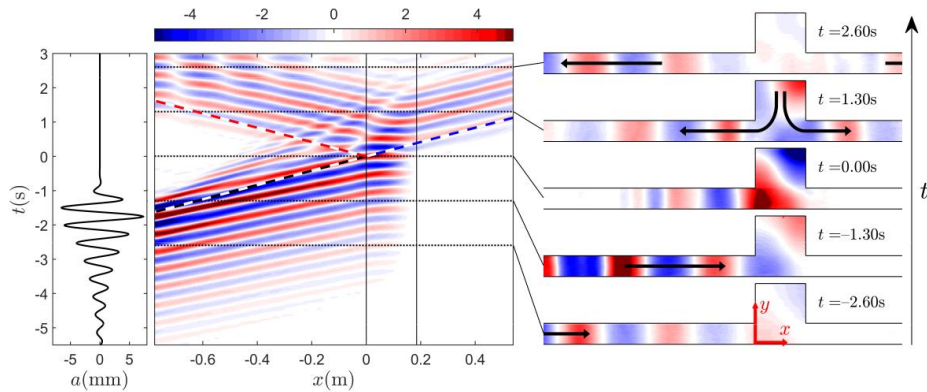
Figure 1: Experimental results. Left: Time signal sent by the wavemaker. Center: Space-time diagram showing the incident wave with no reflection and transmission before the released time t=0 s. The two vertical black line indicates the position of the cavity. Amplitude in mm. Right: Snapshots at different times (black dotted lines in the space-time diagram).
