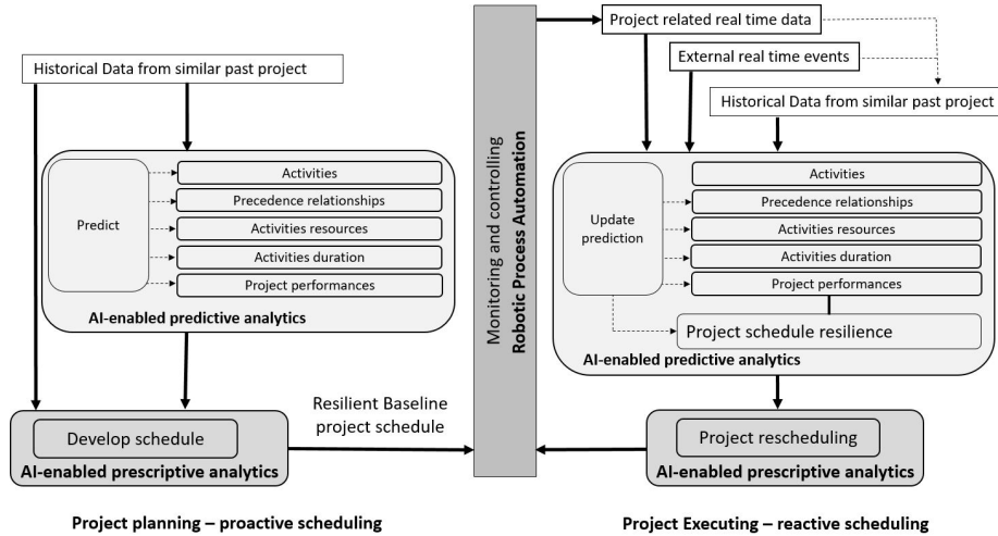
Fig. 1. Framework for building AI-enabled resilient project scheduling
