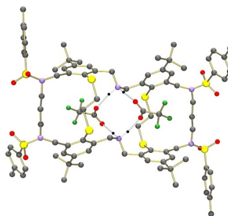
Figure 7. ORTEP view of the X-ray molecular structure of the 1:2 adduct 11·2CF 3 CO 2 H of macrotricyclic 11 and trifluoroacetic acid. Dashed lines represent the bifurcated hydrogen bonds between the trifluoroacetate anions and the protonated bridgehead nitrogen atoms. [29d]
