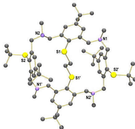
Figure 4. Molecular structure of 7a in crystals of 7a \cdot\text{4CHCl}_3 . Solvent molecules and H atoms omitted for clarity. Symmetry code used to generate equivalent atoms: -x, -y, -z (').
