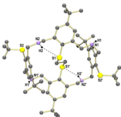
Figure 2. Molecular structure of 6a in crystals of 6a \cdot\text{2MeOH} . H atoms and solvent molecules omitted for clarity. Dashed lines refer to intramolecular hydrogen bonding interactions ( \text{N}2\cdots\text{S}1 3.313(3) Å). Symmetry code used to generate equivalent atoms: -x, -y, -z (').
