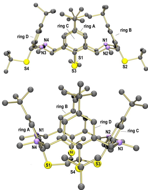
Figure 5. Two views of the molecular structure of 7b in crystals of 7b ·CH 2 Cl 2 . Solvent molecules and H atoms omitted for clarity.
