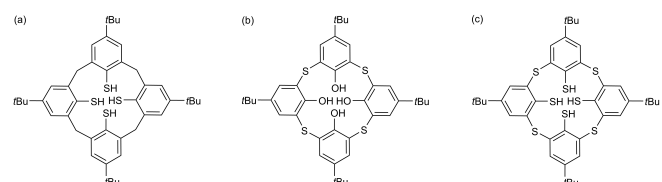
Figure 1. Chemical structures of (a), p - tert -butyltetramercaptocalix[4]arene (b)
