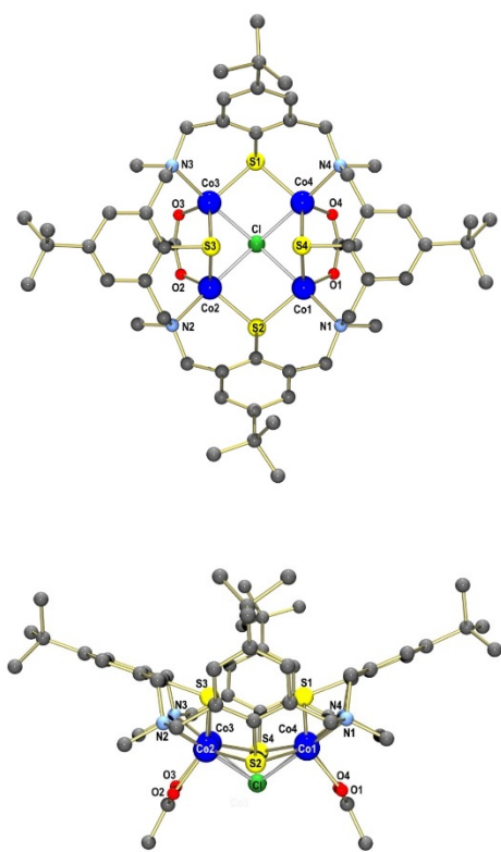
Figure 8. Two views of the molecular structure of the tetranuclear \text{Co}_4 complex 13 .
