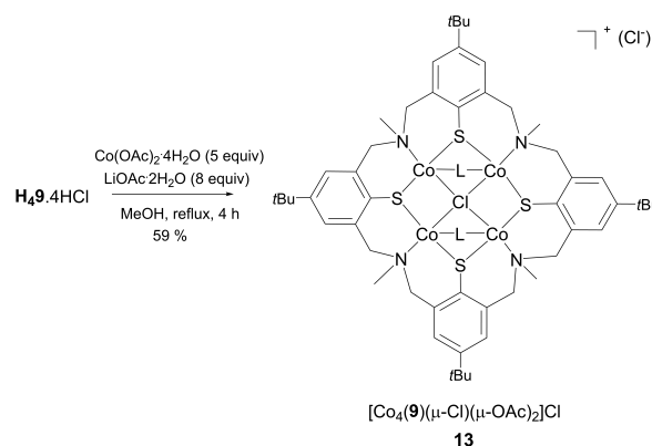
Scheme 4. Synthesis of the tetranuclear cobalt complex 13 .
