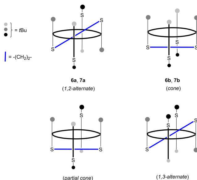
Figure 3. Schematic representation of the molecular structures of four potential isomers of the protected mercaptocalixarenes 6 and 7 . So far, only the 1,2- alternate and cone conformers have been isolated.
