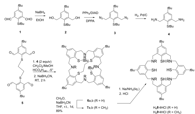
Scheme 1. Synthesis of mercaptothiacalixarenes H 4 8 and H 4 9.
