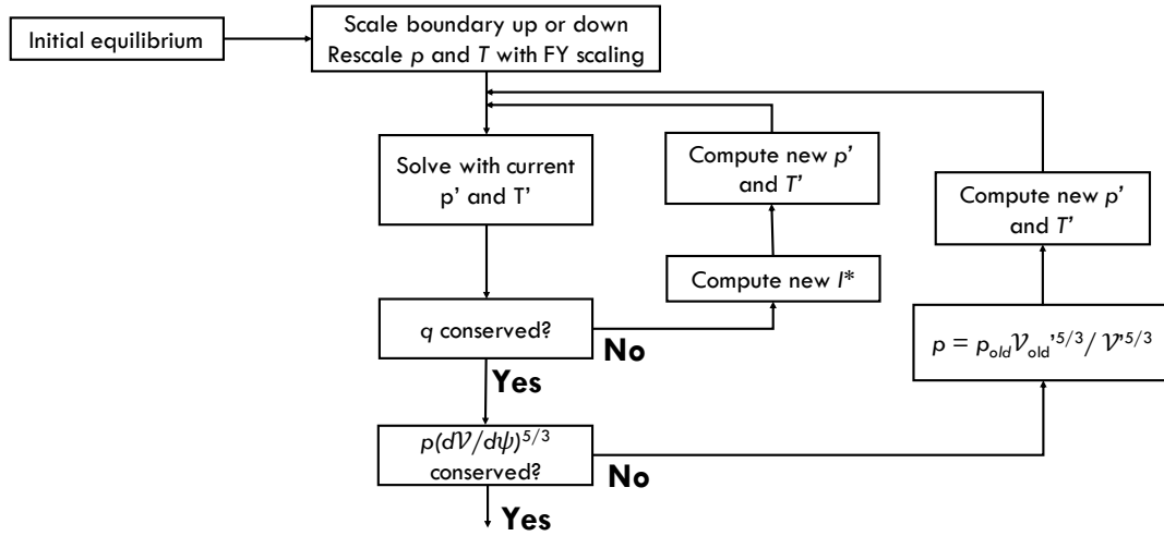
Figure 1. CHEASE workflow for the generation of flux and entropy conserving equilibria.
