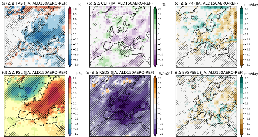
Fig. 10: Mean summer discrepancies in projected climate change signal between ALD150AERO and REF. Dashed areas are statistically significant (see details in Sect. 2.4).
