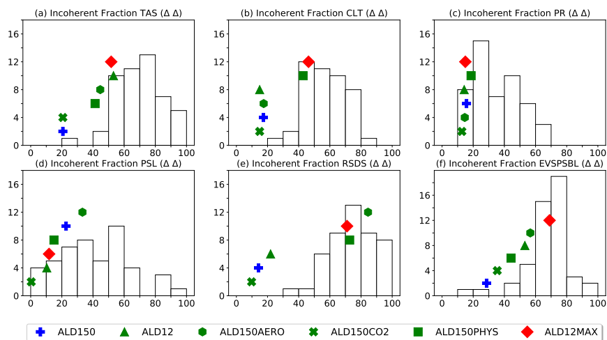
Fig. SM. 13: Fraction of incoherent grid points computed over land part of the standard EUR-11 domain (black box in Article, Fig. 2) for each GCM/RCM pair in the EURO-CORDEX ensemble and each experiment (see methods 2.7) using the discrepancies in winter projected climate change. The fraction is calculated as the ratio between the number of grid points where the differences in projected change for a given variable between REF and ALD are statistically significant and the total number of grid points in the EUR-11 domain. The histograms show the distribution of incoherent fractions in the EURO-CORDEX 48 GCM/RCM pairs, and the fractions for experiments are represented using colored markers with provided legend below the figure.
