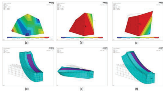
Figure 2 (a) Activation along the diagonal (b) activations along the diagonal and x directions were combined without interaction and (c) with interaction. (d) Beam model with a central muscle having fibers along beam axis, (e) diagonally oriented fibers and with (f) two families of orthogonal fibers.
