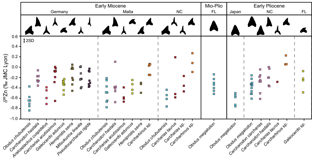
Fig. 2 Zinc isotope ( \delta^{66}\text{Zn} ) composition of fossil elasmobranch enameloid. Teeth are from the Early Pliocene of Japan, North Carolina (NC) and Florida (FL), Pliocene to Miocene transition of Florida, the Early Miocene of North Carolina, Germany and Malta. For more details on the sample background, see Supplementary Data 1, Supplementary Note 2. Silhouettes are not to scale. Measurement uncertainty is indicated at the 2 SD level. Samples are colour-coded following their genus, regardless of locality. Source data are provided as a Source Data file.
