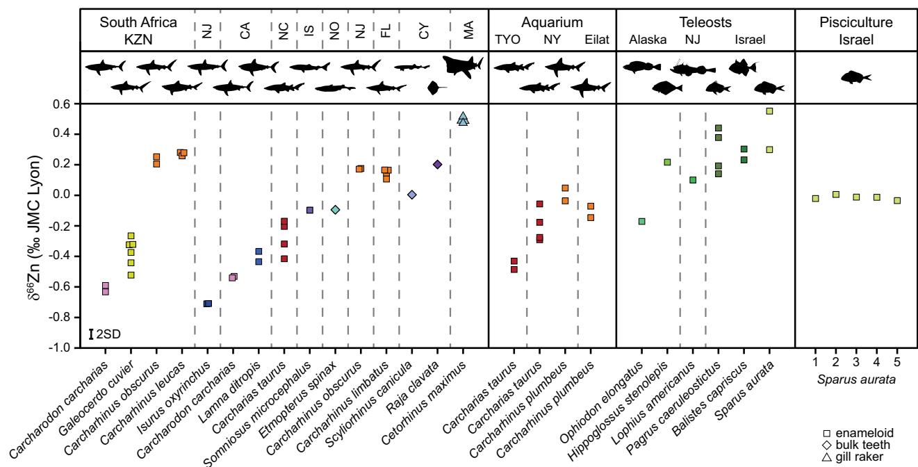
Fig. 1 Zinc isotope ( \delta^{66}\text{Zn} ) composition of extant elasmobranch and teleost fish teeth and gill raker. Specimens come from off the coast of KwaZulu-Natal (KZN) South Africa, New Jersey (NJ), California (CA), North Carolina (NC), Iceland (IS), Norway (NO), Florida (FL), Cyprus (CY), Massachusetts (MA), Alaska and Israel. Aquarium sharks are from the New York (NY) and Tokyo (TYO) Aquariums and the Eilat (Israel) Underwater Observatory Park. Pisciculture S. aurata individuals are numbered and plotted individually to visualise the homogeneity among control-fed individuals compared to wild elasmobranchs and teleosts. Silhouettes are not to scale. Measurement uncertainty is indicated at the 2 SD level. Samples are colour-coded following their genus, regardless of locality. Source data are provided as a Source Data file.
