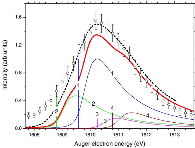
FIG. 1. Calculated line shape of the L_2 - M_{4,5}N_{2,3} Auger transition at \Delta E = 4 eV photon excess energy above the 1s ionization threshold. Thin colored lines marked as 1–4 show contributions of individual transitions (see text). Thick vertical lines show the locations of these lines and their relative strengths. The thick red line shows the summed calculated line shape and the dashed line presents this intensity convoluted with the electron detector resolution function. The black open circles present the measured spectrum at the same energy.
