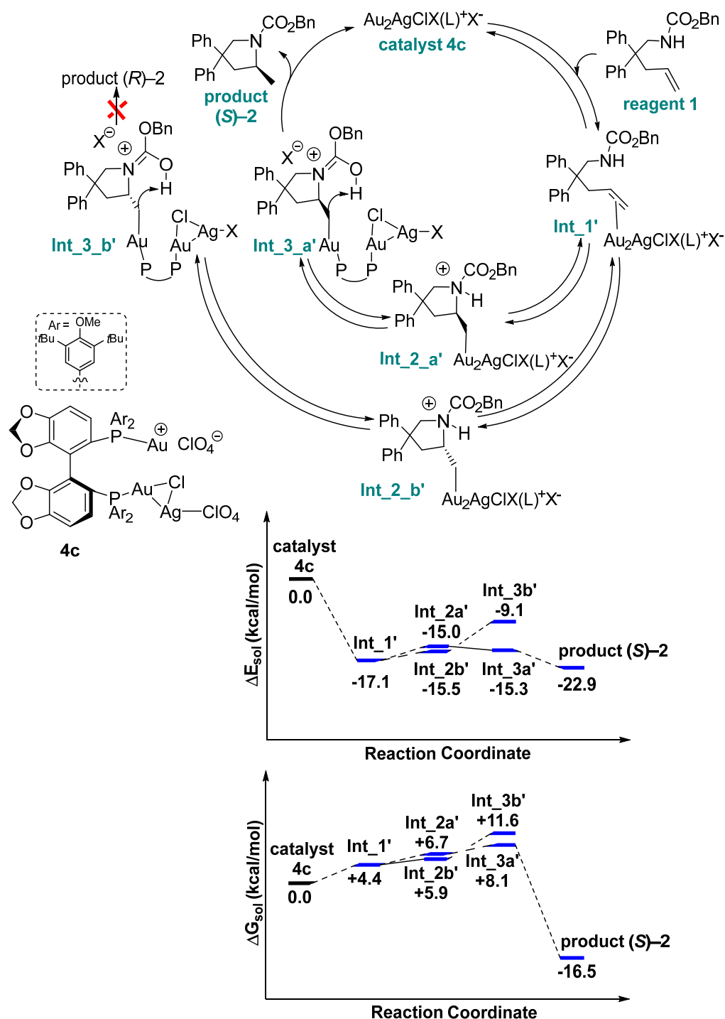
Figure 4. The proposed reaction mechanism for the formation of the amine product ( S )-2 in methanol using catalyst 4c , and without the assistance of one methanol molecule. The electronic energy profile is shown at PBE0/def2-TZVP//PBE/def-TZVP level of theory. All values are in kcal/mol.
