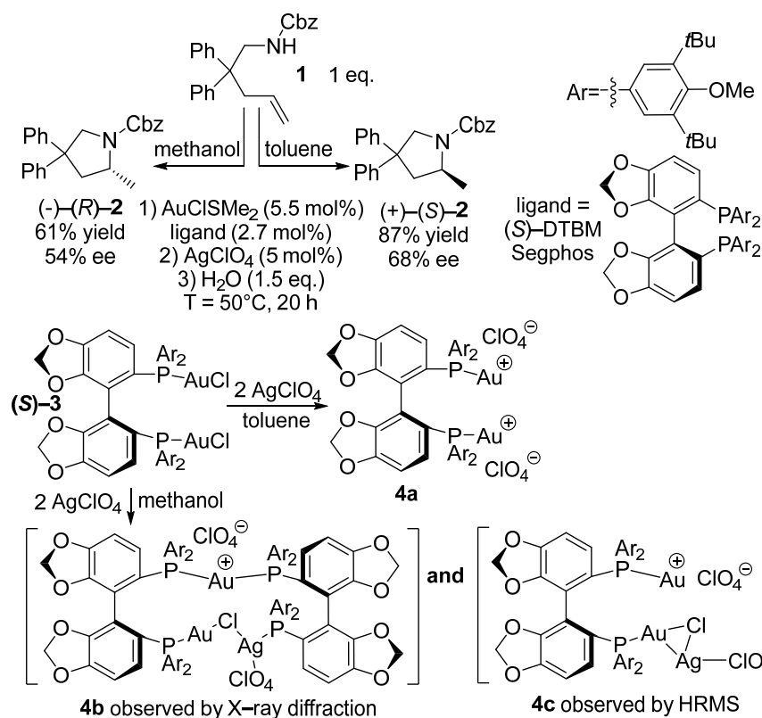
Scheme 1. Enantiodivergent intramolecular hydroamination of alkenes catalysed by gold(I) cationic complex and preparation of gold(I) cationic complexes 4a , 4b and 4c .
