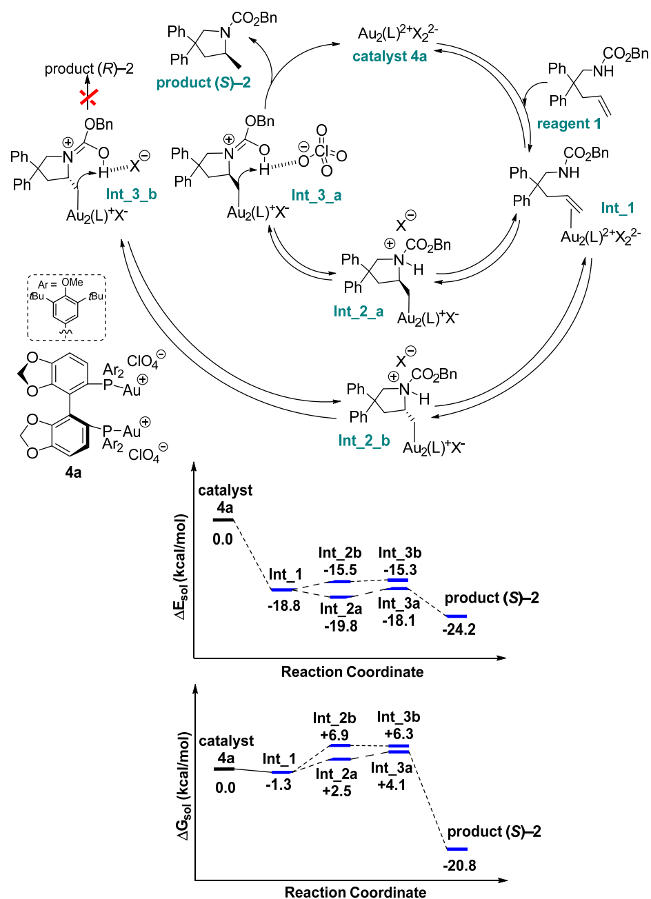
Figure 1. The proposed reaction mechanism for the formation of the amine product ( S )-2 in toluene using catalyst 4a . The electronic energy profile is shown at PBE0/def2-TZVP//PBE/def-TZVP level of theory. All values are in kcal/mol.
