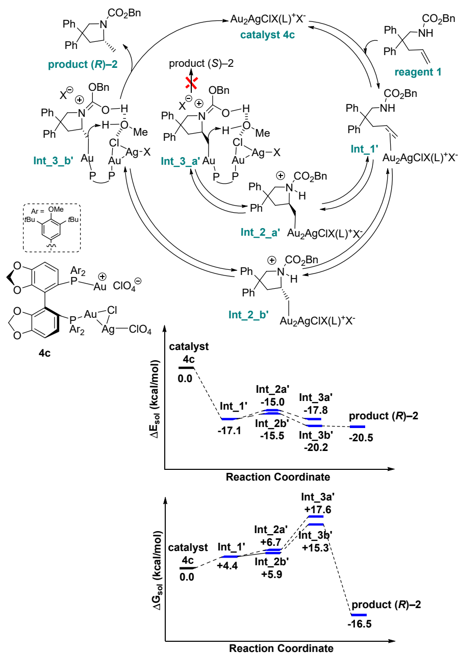
Figure 2. The proposed reaction mechanism for the formation of the amine product ( R )- 2 in methanol using catalyst 4c ; calculations at the PBE0/def2-TZVP//PBE/def-TZVP level of theory with DFT. All values are in kcal/mol.
