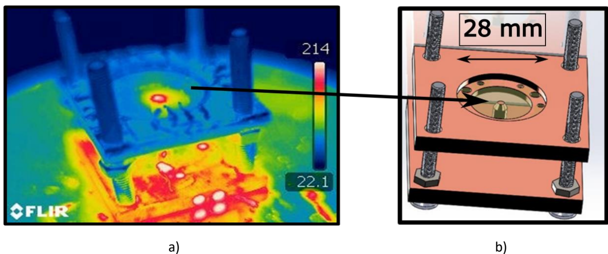
Figure 5 : Thermal view of the device for a temperature gradient of around 200K (a) and associated scheme (b)
