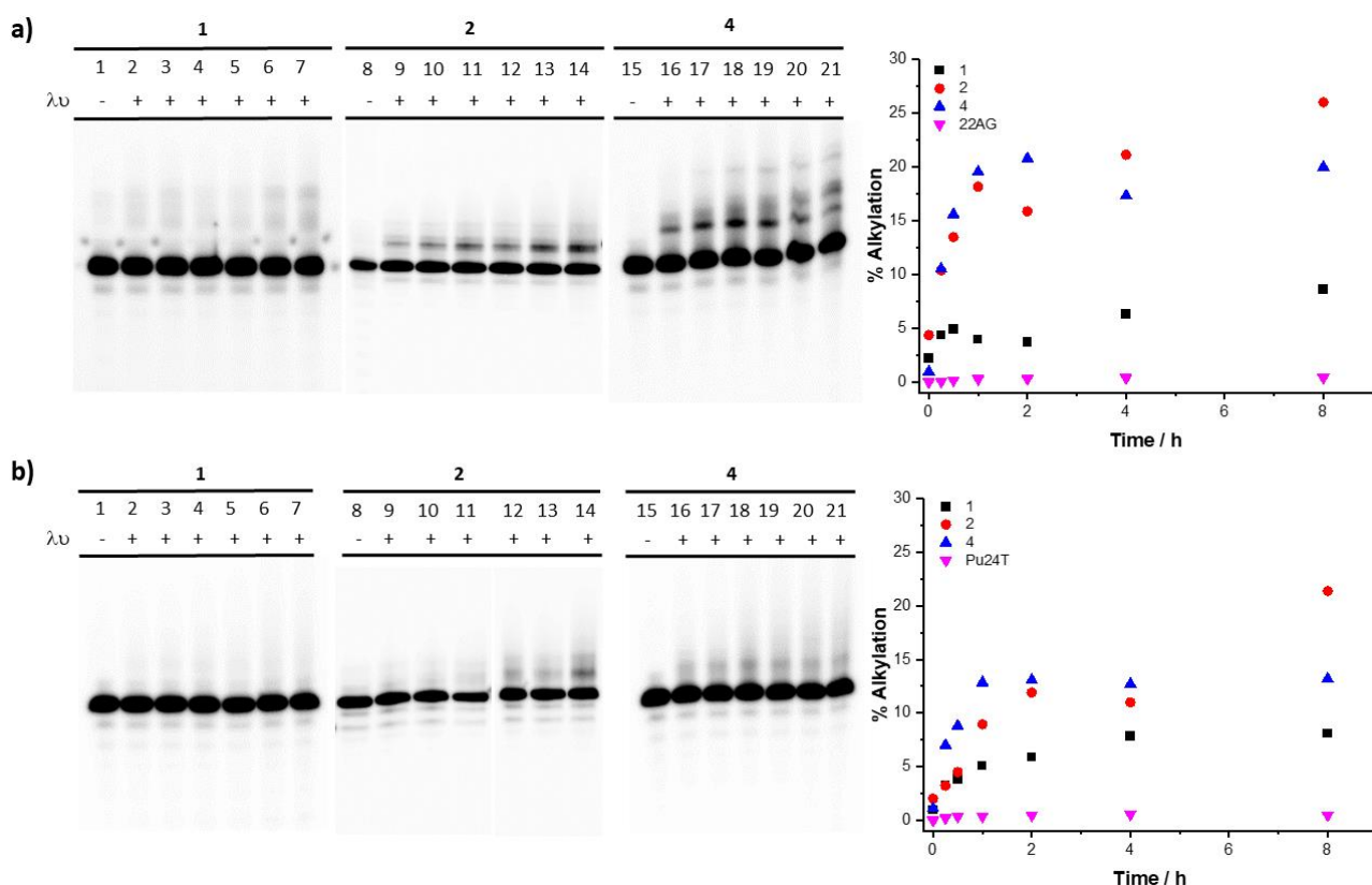
Figure 6. Denaturing gel electrophoresis (15% acrylamide) of the alkylation products of (a) 22AG and (b) Pu24T (10 \mu M) in the presence of K + buffer (10 mM Li Caco (pH 7.2), 100 mM KCl) with 1 , 2 , and 4 (20 \mu M) at increasing irradiation time (0, 0.25, 0.5, 1, 2, 4, and 8 hrs). Lanes 1, 8, and 15 are control experiments showing the effect in the absence of irradiation with (a) 22AG and (b) Pu24T. Lanes 2 - 7 show the results of irradiation of 22AG and Pu24T at 365 nm in the presence of 2 equivalents of 1 , lanes 9 - 14 show the results of irradiation of 22AG and Pu24T at 365 nm
