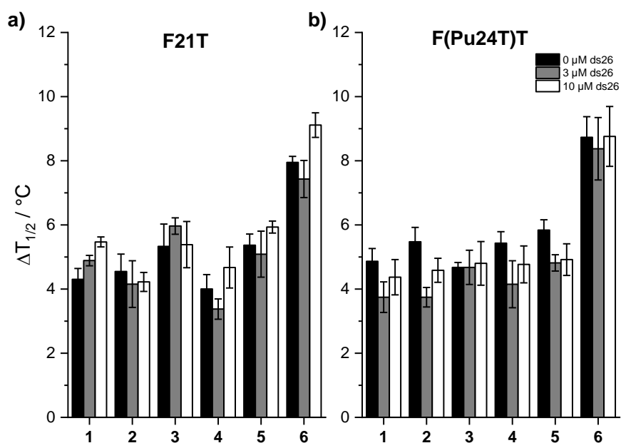
Figure 3. FRET-melting competition assay with (a) F21T and (b) F(Pu24T)T in the absence and in the presence of double-stranded DNA competitor (ds26). Conditions: F21T or F(Pu24T)T 0.2 \mu\text{M} , compounds 2 \mu\text{M} , ds26 0, 3, or 10 \mu\text{M} (black, dark gray and white bars, respectively) (a) Li Caco 10 mM (pH 7.2), LiCl 90 mM and KCl 10 mM and (b) Li Caco 10 mM (pH 7.2), LiCl 99 mM and KCl 1 mM. Analyzed compounds 1-6 .
