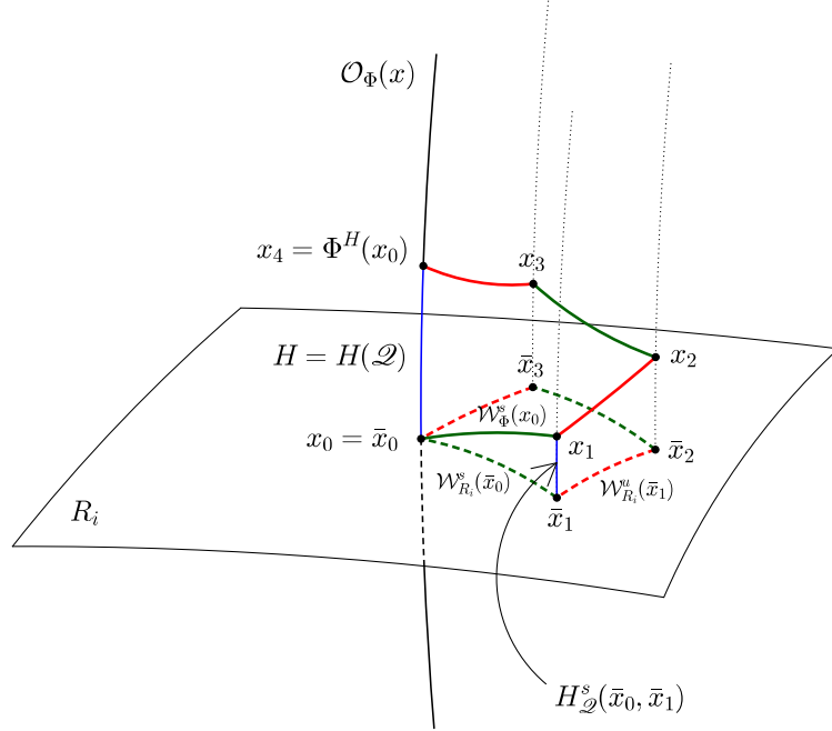
FIGURE 3. Quadrilaterals and temporal displacements.
