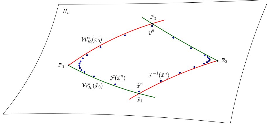
FIGURE 4. Shadowing periodic orbits with a prescribed combinatorics.
