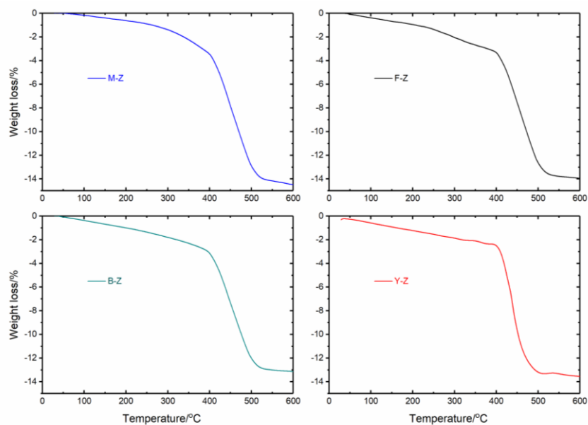
Figure 7. TGA curves of the inter-zeolite transformation products in the acidic medium.
