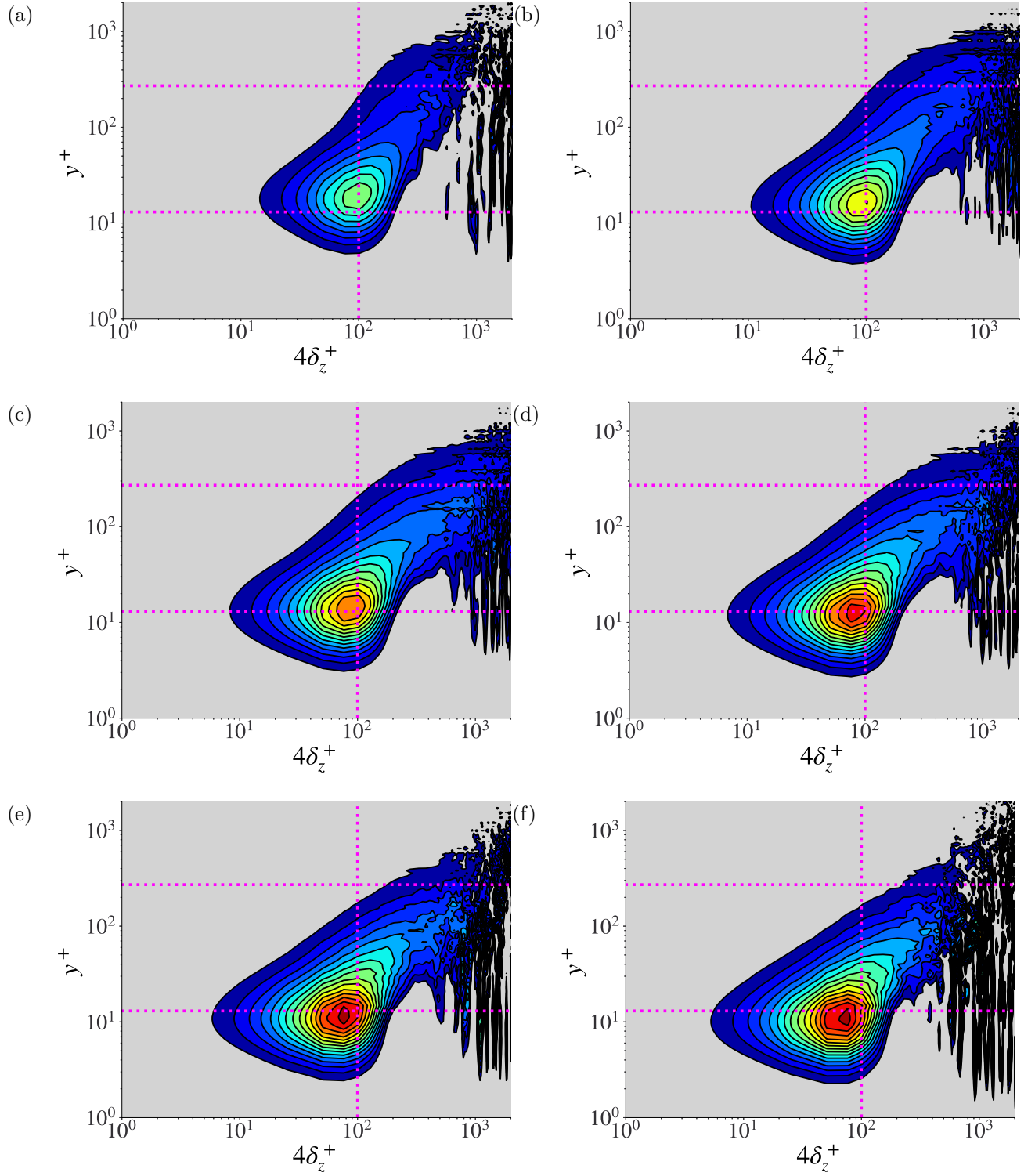
FIG. 13: Maps of \delta z \frac{dS_u^2(\delta z)}{d\delta z} \Big|_{CfLS}^+ in the y^+ - \delta z^+ plane conditional on the six Cf_{LS} shown in figure 7; (a)-(f) arranged in order of rising Cf_{LS} values.
