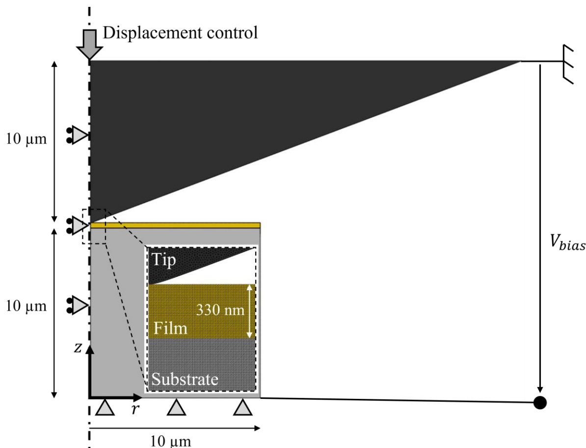
Figure S4. Numerical model for the FEM simulations.
