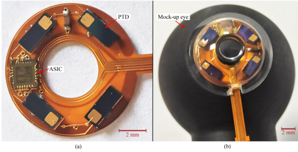
Fig. 5. Prototype SCL fabricated embedding the ASIC and 4 PTDs.
