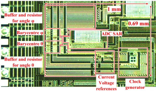
Fig. 4. Microphotograph of the eye tracking circuit implemented in a multi-projects die.
