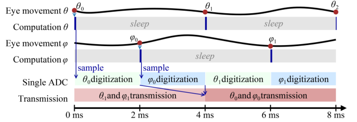
Fig. 3. Timing diagram for the proposed system. Barycenter computing units continuously compute \theta_{\text{computed}} and \varphi_{\text{computed}} which are sequentially digitized at 500 Hz.
