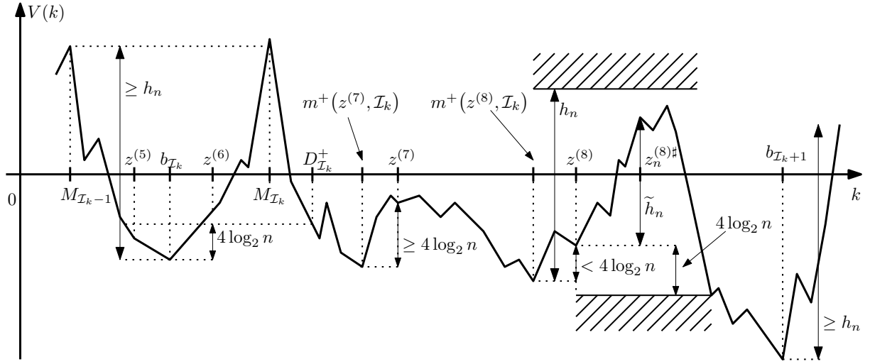
Figure 8. Schema of the potential V , with z represented as z^{(5)} in the first case of the proof of Lemma 5.12, z^{(6)} in the second one, and as z^{(7)} on E_{21,k}^{(n,z)} and z^{(8)} on E_{22,k}^{(n,z)} for the proof of Lemma 5.13.
