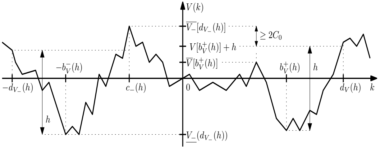
Figure 3. Schema of the potential V for the first case of the proof of Lemma 2.12 when \bar{V}[b_V^+(h)] < V[b_V^+(h)] + h .
