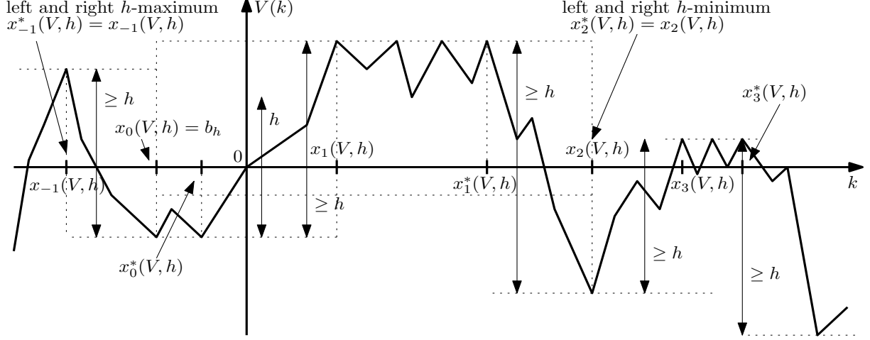
Figure 1. Schema of the potential V with left h -extrema x_i(V, h) (defined before (19)) and right h -extrema x_i^*(V, h) (defined before (45)).
