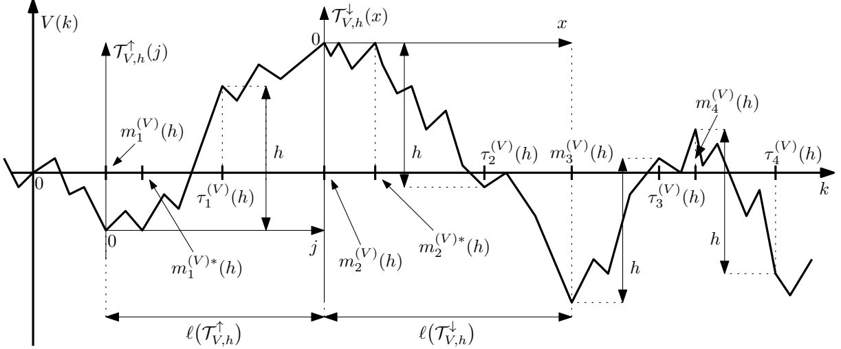
Figure 2. Schema of the potential V with the \tau_i^{(V)}(h) , m_i^{(V)}(h) , \mathcal{T}_{V,h}^\uparrow , \mathcal{T}_{V,h}^\downarrow and m_i^{(V)*}(h) .
