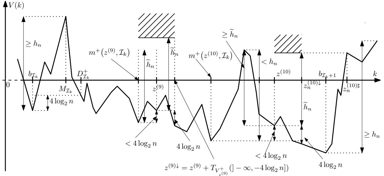
Figure 9. Schema of the potential V , with z equal to z^{(9)} on E_{23,k}^{(n,z)} \cap E_{27,k}^{(n)} , and z^{(10)} on E_{23,k}^{(n,z)} \cap (E_{27,k}^{(n)})^c .
