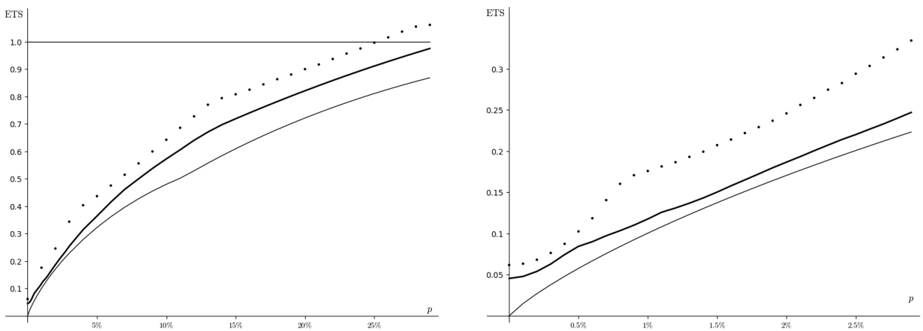
Figure 4: Comparison between the best hypercube designs (dots) and the best identified designs selected (thick curve). The thin curve gives the best known lower bound.
