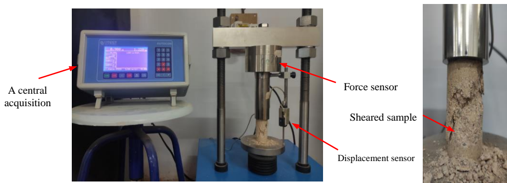
Figure 4. UCS test loading steps
