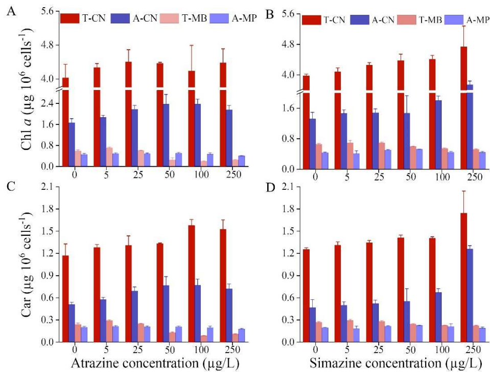
314 315 Figure 2. The effects of atrazine (A, C) and simazine (B, D) on the pigment contents of 316 four species, including (red color) temperate C. neogracile (T-CN) and temperate M. 317 bravo (T-MB), (blue color) Arctic C. neogracilis (A-CN) and Arctic M. polaris (A-MP) 318 after 72 h exposure. Data are expressed as means ± SD (n = 6).
