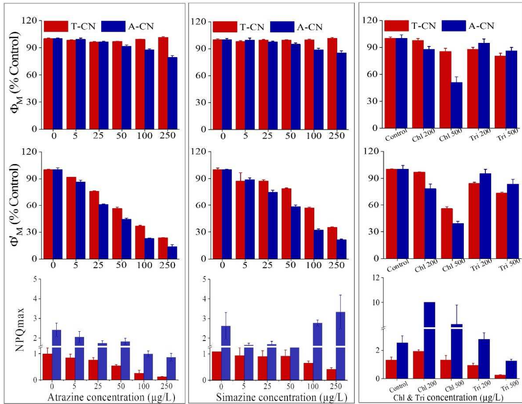
341 Figure 3. The effects of atrazine, simazine, chlorpyrifos and trifluralin on the maximal 342 PSII quantum yield ( \Phi_M ) and the operational PSII quantum yield ( \Phi'_M ) of temperate C. 343 neogracile (red color-T-CN) and Arctic C. neogracililis (blue color-A-CN) after 72 h 344 exposure. Chl and Tri represent chlorpyrifos and trifluralin respectively. Data are 345 expressed as means \pm SD (n = 6).
