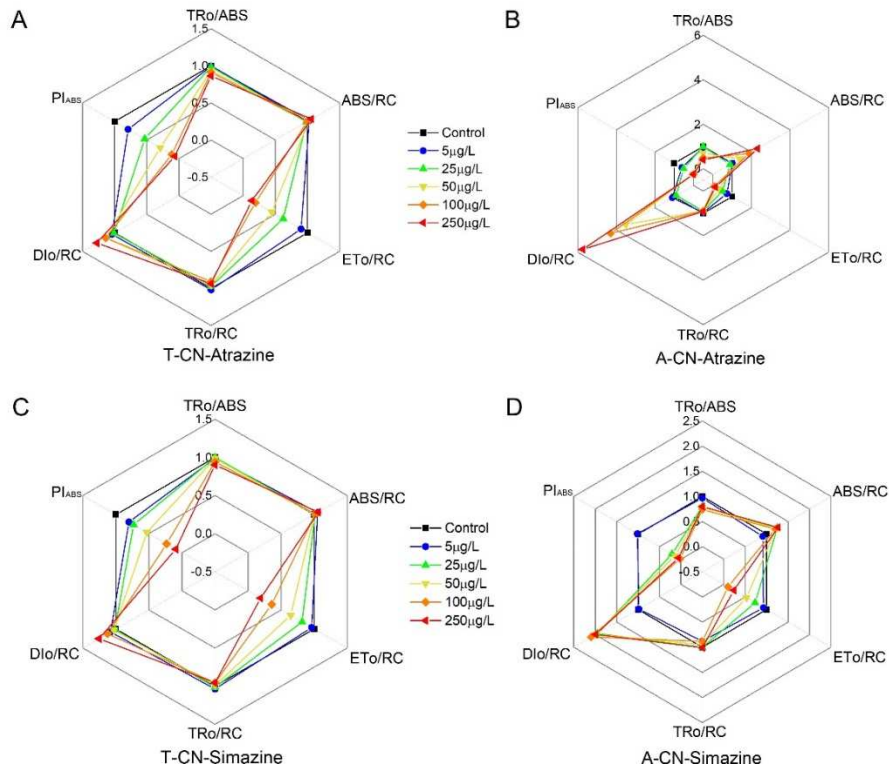
381 Figure 5. The effects of atrazine and simazine on the chlorophyll fluorescence 382 parameters of temperate C. neogratile (T-CN) and Arctic C. neogracilis (A-CN) after 383 72 h exposure.
