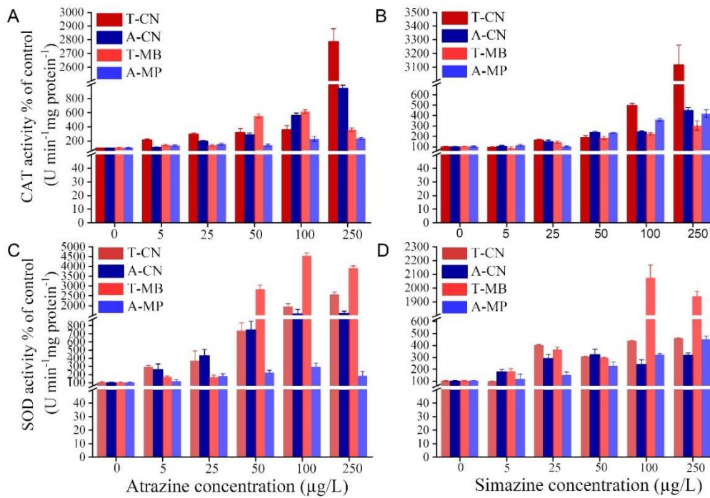
433 Figure 8. The effects of atrazine (A, C) and simazine (B, D) on the catalase (CAT) and 434 superoxide dismutase (SOD) of four species, including (red color) temperate C.
