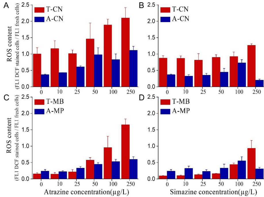
428 Figure 7. The effects of atrazine (A, C) and simazine (B, D) on the reactive oxygen 429 species (ROS) of four species, including (red color) temperate C. neogracile (T-CN) 430 and temperate M. bravo (T-MB), (blue color) Arctic C. neogracilis (A-CN) and Arctic 431 M. polaris (A-MP) after 72 h exposure. Data are expressed as means \pm SD (n = 6).
