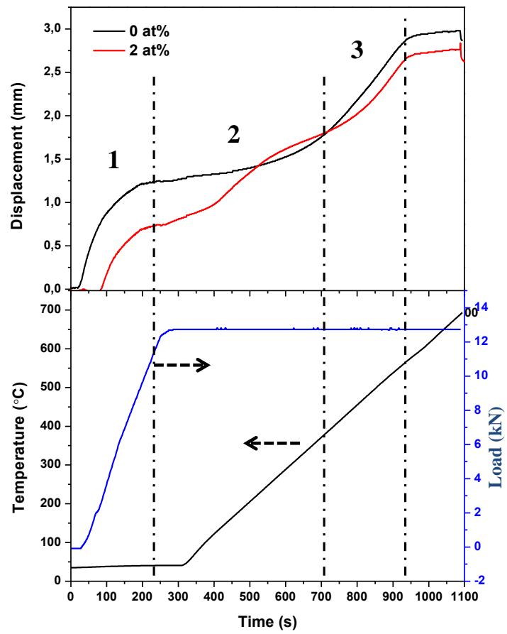
Fig.1 Sintering behavior of pure ZnO and Al-doped ZnO using spark plasma sintering
