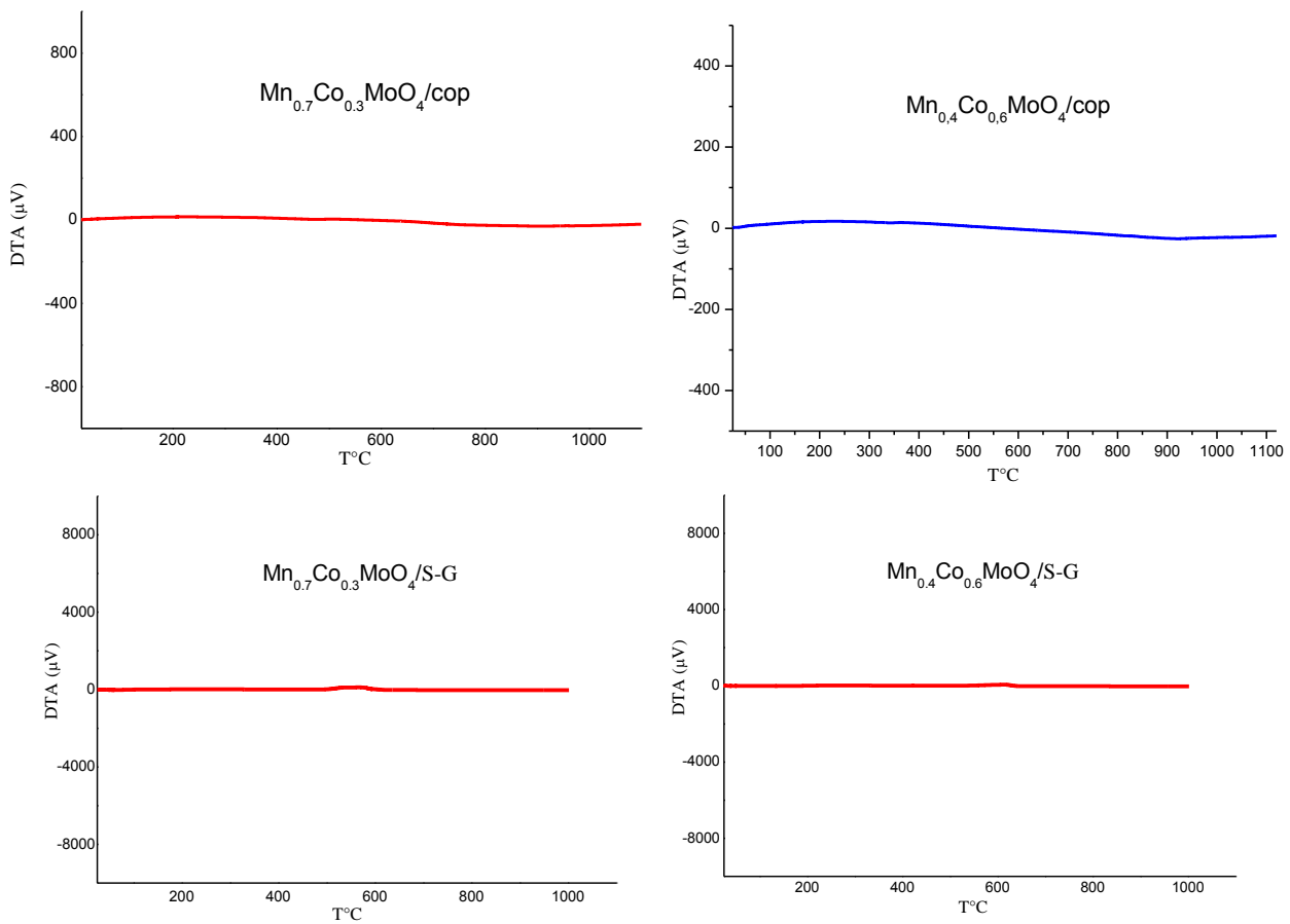
Fig.13. DTA analysis of Mn_{0.7}Co_{0.3}MoO_4 and Mn_{0.4}Co_{0.6}MoO_4 powders obtained by sol-gel route at 700°C (S-G) and by co-precipitation at 500°C (Cop).
