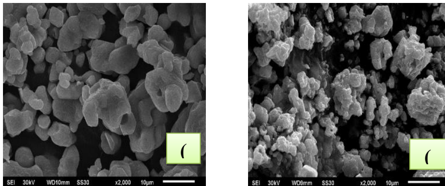
Fig. 8. SEM micrographs of \text{Mn}_{1-x}\text{Co}_x\text{MoO}_4 powders (a): x = 0.3 and (b): x = 0.6 prepared by sol-gel route.
