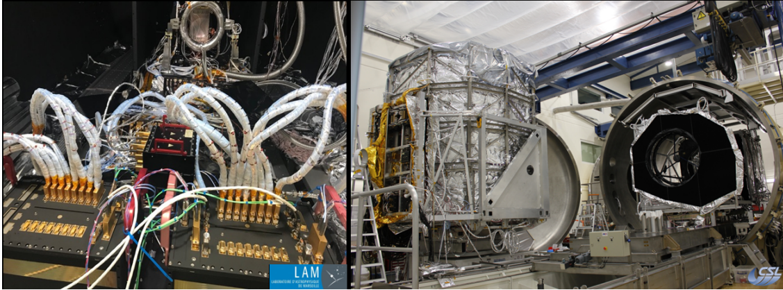
Figure 8. Left : NISP tests setup at Laboratoire d'Astrophysique de Marseille , France. NISP warm electronics close-up, from bottom to top: the two DPUs, the ICU, and the focal plane array. Right : Euclid's end-to-end PLM test setup at the Centre Spatial de Liège , Belgium. The NISP warm electronics mounted on the panel Y can be seen at the left-side of the picture (vertical structure partially covered with MLI), and the telescope placed horizontally at the right-side of the image.
