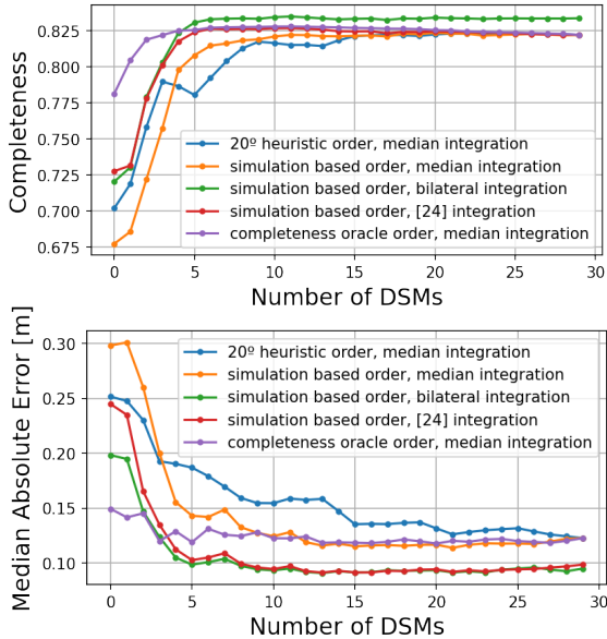
Figure 5. Progressive integration of DSMs for region JAX_156. Completeness (top) and MAE (bottom) evolution when integrating a growing number of DSMs. Purple curve corresponds to an integration by the median and an oracle ordering. Curves in blue, orange and green correspond to the C1, C2 and C3 configurations of the pipeline respectively. Red curve corresponds to an implementation of the method in [24]. Refer to the text for a complete description.
