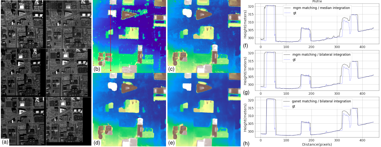
Figure 1. (a) Six images of a region of the Omaha dataset. (b) Ground truth (GT) height map of the region. MVS reconstructions using all 30 stereo pairs: (c) DSMs computed using the MGM [10] correlator and integrated by the median of the DSMs, (d) DSMs computed using the GANet [28, 13] correlator and integrated by the median of the DSMs, (e) DSMs computed using the GANet correlator and integrated by bilateral filtering. Profiles corresponding to the red line: (f) from images b and c, (g) from images b and d, (h) from images b and e.
