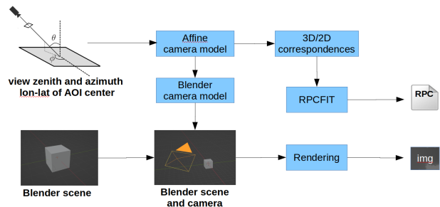
Figure 2. Block diagram of the simulator. Please refer to the text for the description of the blocks and the flow of data.
