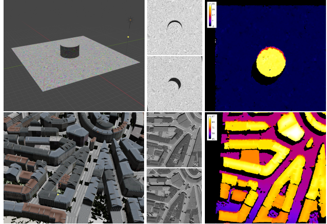
Figure 3. Results of the simulation tool with two different 3D scenes. From left to right: a view of the 3D scene, a stereo pair generated with the simulation tool, and the DSM reconstructed with the S2P pipeline. Above: Cylinder scene. The scene is composed of a cylinder with a radius of 25m and a height of 30m. Surfaces have a random texture. Below: Artificial city scene.
