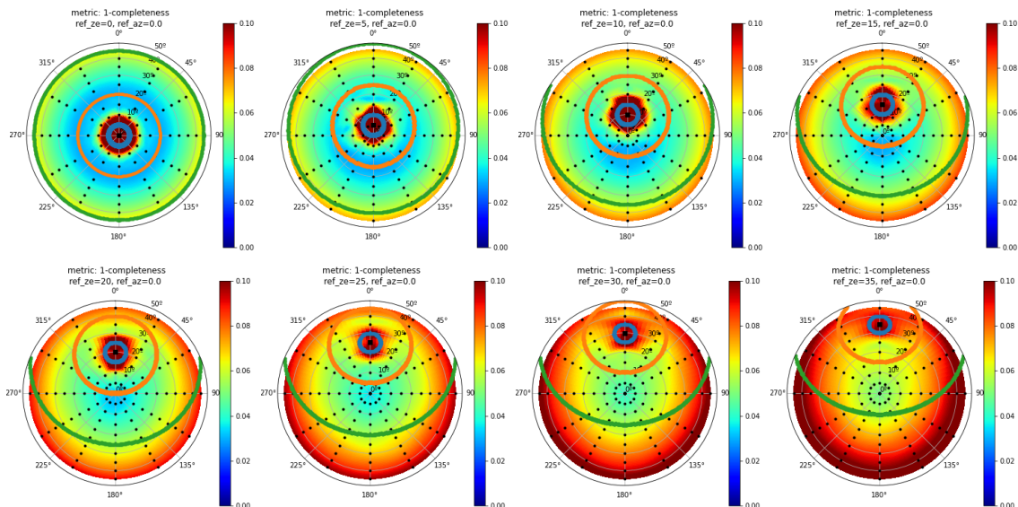
Figure 4. Reconstruction errors of simulations for different reference-secondary image orientations. The square represents the reference view and circular points represent the tested secondary views. Metric 1-COMP is shown for increasing zenith angle of the reference view. Blue corresponds to small errors while red indicates large errors. The blue, orange and green curves indicate the positions in the hemisphere for views 5°, 20° and 45° apart from the reference, respectively.
