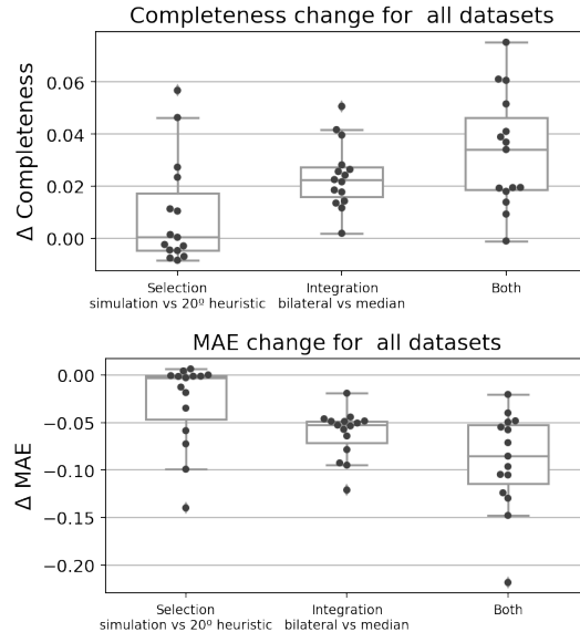
Figure 6. Incremental results between configurations C1, C2 and C3 (see text). For each region in the datasets, the top 5 DSMs are integrated and the resulting DSM compared to the GT. Left: C2 - C1 (pair selection by simulation vs. heuristics), Center: C2 - C1 (integration by bilateral filter vs. integration by the median). Right: C3 - C1 (both improvements vs. the original baseline pipeline). Note how each contribution increases the global performance.
