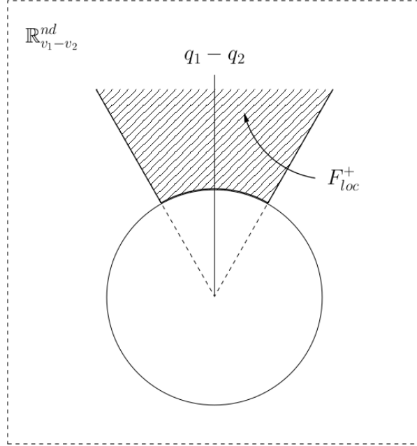
Figure 2.1: Fiber over q_1 - q_2 of \tilde{F}_{\text{loc}}^+ in the n = 2 case
