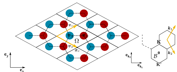
Figure 1: Honeycomb media in the case of disk shaped inclusions (left). Dual lattice \Lambda^* , hexagonal Brillouin zone \mathcal{B} , dual basis (\mathbf{k}_1, \mathbf{k}_2) and high symmetry quasimomenta \mathbf{K} and \mathbf{K}' (right).
