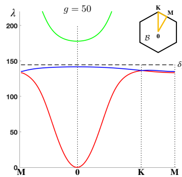
Figure 2: \mathbf{k} \mapsto \lambda_1(\mathbf{k}; 50) , \lambda_2(\mathbf{k}; 50) , \lambda_3(\mathbf{k}; 50) plotted along the (yellow) contour: \mathbf{M} - \mathbf{0} - \mathbf{K} - \mathbf{M} of \mathcal{B} for disks inclusions of radius R = 0.2 .
