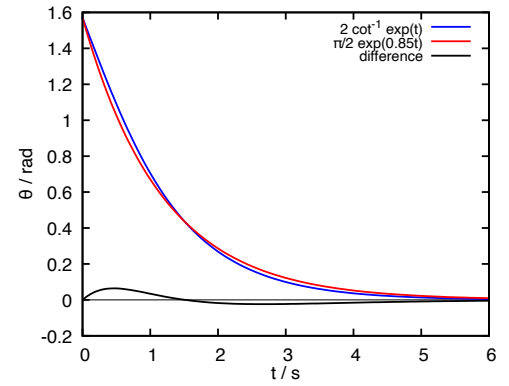
FIG. 17. Approximation by an exponential function of the exact solution to the differential equation for the rotation of the bacterium as a function of time, see Eq. (5). The optimal fit is for a prefactor 0.85(1), in which case the error is less than 0.065 rad.
