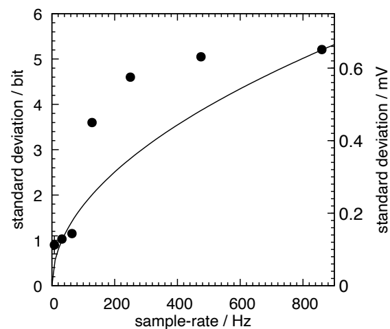
FIG. 8. Standard deviation (RMS noise) over 1000 samples taken by the AD converter of the detector photodiode signal as a function of sample rate. Noise increases with increasing sample rate, but not proportional to the square root of the bandwidth (solid line). There is a strong increase in noise above 64 samples/s.
