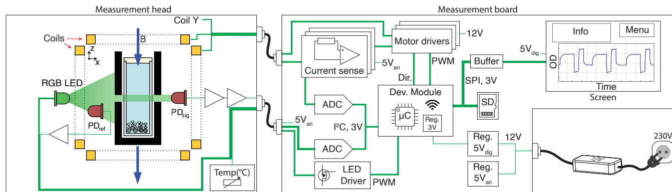
FIG. 4. Diagram of the system: Measurement head: LED, reftiode, diode, amplifier stages, coils, cuvette, bacteria. Measurement board: outlet to 12 supply, 12 V to 5 V analog and digital, microcontroller, AD converter, LED driver, motor shields, current sense, HDMI cable, coil cable, SD card, WiFi. User interface: resistive touchscreen. Measurement board and user interface reside in the same housing.
