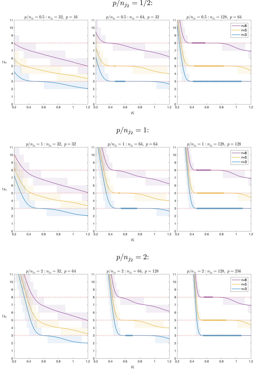
Figure 3: The asymptotic performance of \hat{r}(j_1, j_2, \kappa) . Each plot displays \hat{r} versus \kappa based on 5000 observations of \{\Delta_1(j_1, j_2), \dots, \Delta_p(j_1, j_2)\} for p/n_{j_2} \in \{0.5, 1, 2\} (top to bottom, respectively), over sample sizes n \in \{2^{10}, 2^{12}, 2^{14}\} (left to right column, respectively). The solid lines represent the Monte Carlo average for the particular choice of r, n and p . The upper/lower limits of shaded regions correspond the empirical regions between quantiles 0.05 and 0.95. The marked lines (with small “x” markers) are the points at which the mean was exactly equal to the corresponding value of r .
