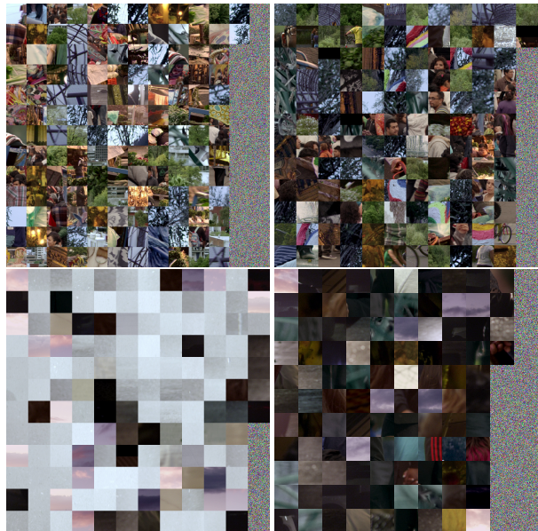
Fig. 3: Examples of tube-contents from 4 clusters, each tube-content reference tube is represented, noise pattern is used as right-padding to square visualizations. Top clusters tend to capture high spatial and temporal frequency texture, while bottom clusters model more flat or darker textures.
